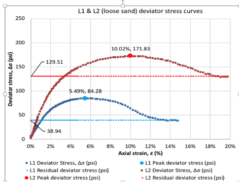
Figure 1: Deviator stress curves for sample 1 and 2
