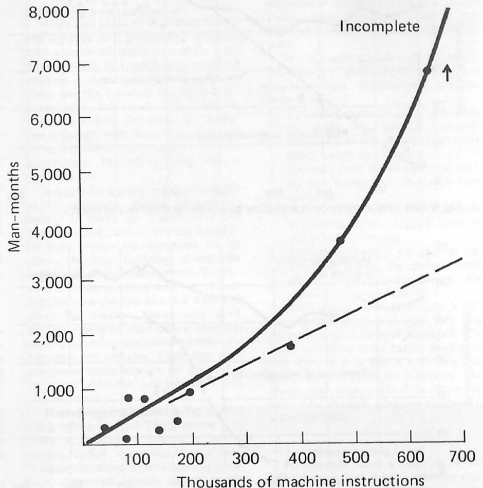
Fig. 5. As a project's complexity increases, the number of man-months required to complete it goes up exponentially.
