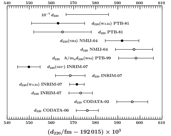
FIG. 1 Inferred values (open circles) of d_{220} from various measurements (solid circles) of d_{220}(X) . For comparison, the 2002 and 2006 CODATA recommended values of d_{220} are also shown.
