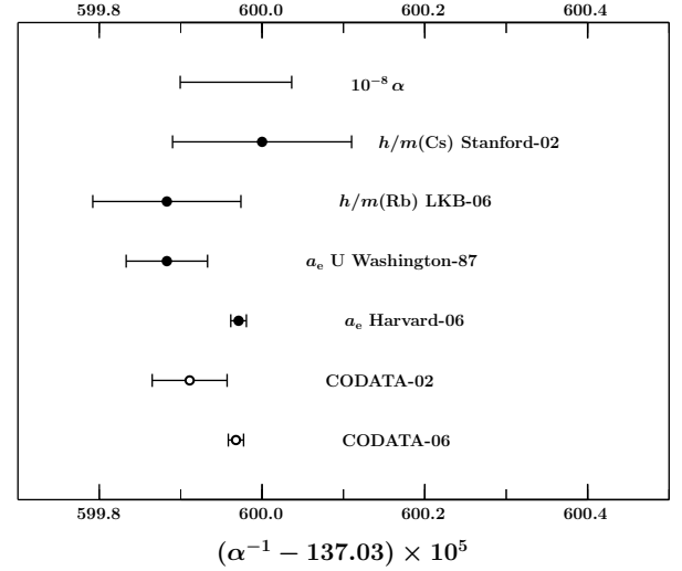
FIG. 4 Values of the fine-structure constant \alpha with u_r < 10^{-8} implied by the input data in Table XXX, in order of decreasing uncertainty from top to bottom. (See Table XXXIV.)
