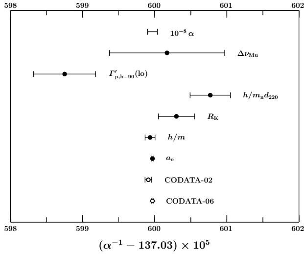
FIG. 5 Values of the fine-structure constant \alpha with u_r < 10^{-7} implied by the input data in Table XXX, taken as a weighted mean when more than one measurement of a given type is considered [see Eqs. (361) to (366)], in order of decreasing uncertainty from top to bottom.
