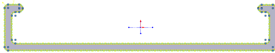
Figure 3.6 Adjusting wall thickness of the profile to account for die swell.
