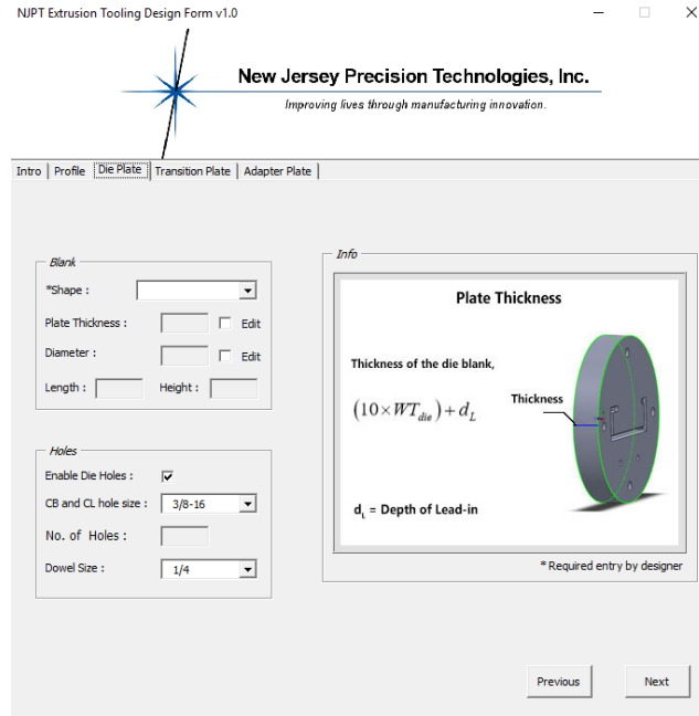
Figure 4.5 Page of extrusion tooling design form GUI that deals with Die plate.
