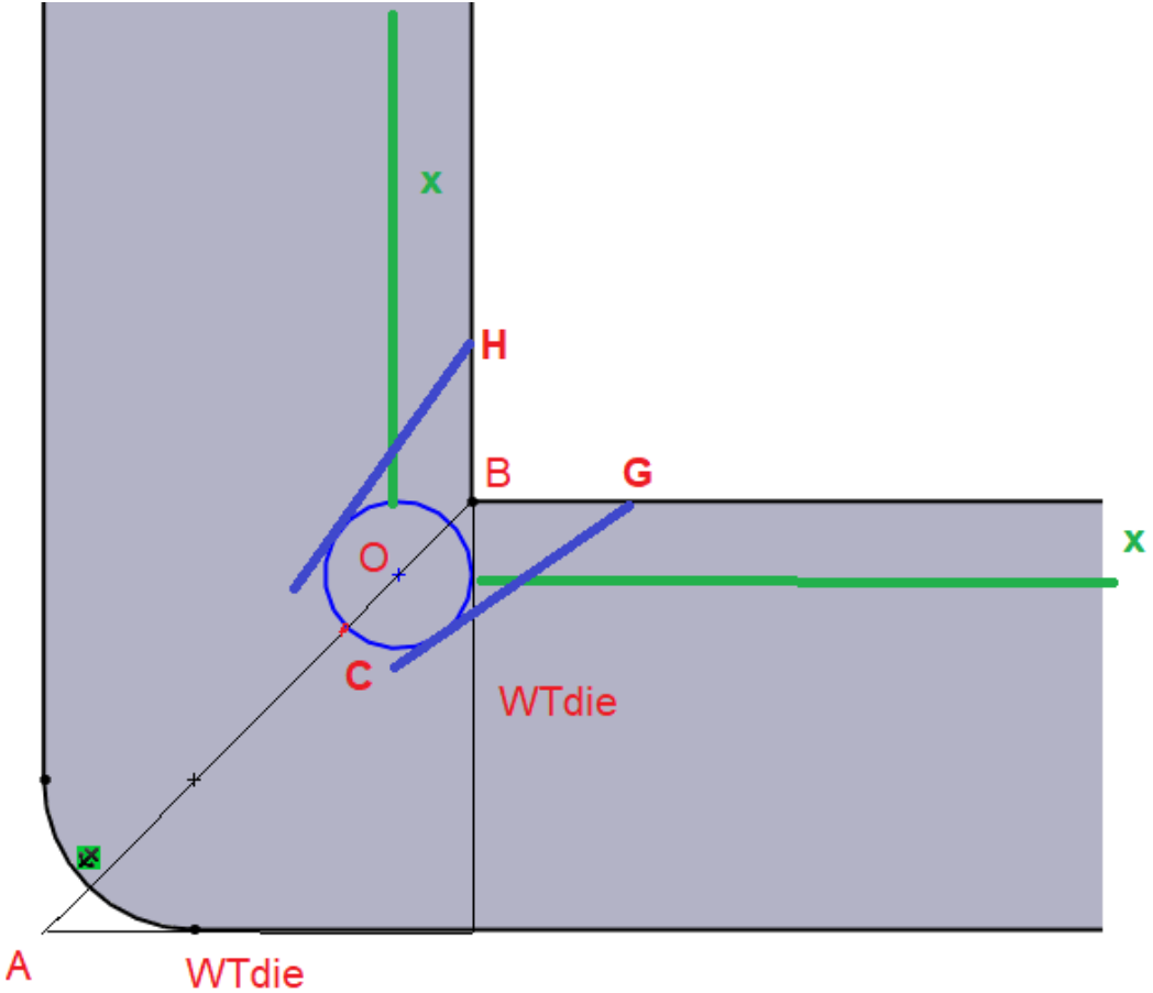
Figure 4.21 Routine steps for creating a flow restrictor at the joints of a profile.
