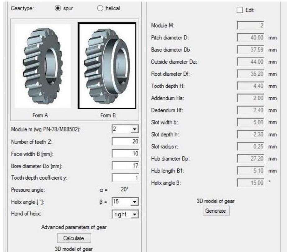
Figure 1.9 Automated design system used for gear generation.
