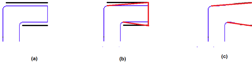
Figure 4.20 Leg modifications for a Type 1 leg with length less than 3/8 in and having only flares, (a) Sides of the leg are offset sideways to add flares, (b) Lines are joined at the points of intersections and base points of the leg, (c) Unwanted lines are trimmed to get the modified leg.
