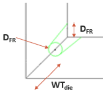
Figure 3.20 Dimensions of a flow restrictor found at the joints of an extrusion profile.
