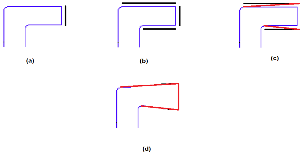
Figure 4.18 Leg modifications for a Type 1 leg with length less than 3/8 in and having flares and extensions, (a) The outer edge is extended outwards, (b) Sides of the leg are offset sideways to add flares, (c) Lines are joined at the points of intersections and base points of the leg, (d) Unwanted lines are trimmed to get the modified leg.
