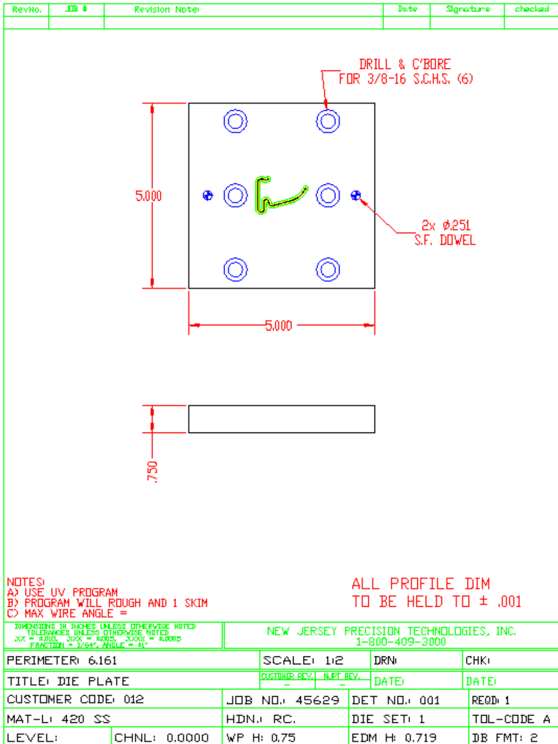
Figure C.7 Drawing sheet generated for Job 45629 depicting Die plate.
