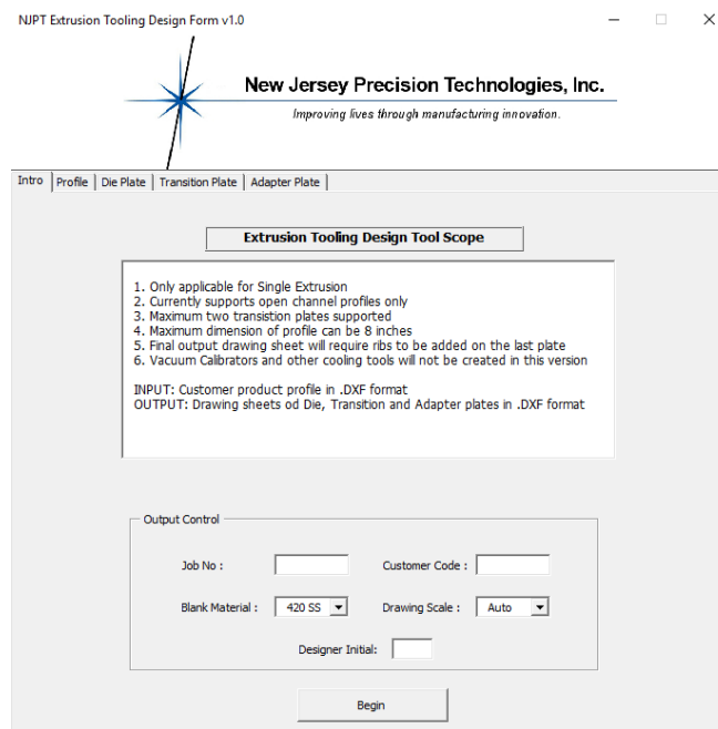
Figure 4.2 Intro page of the main extrusion tooling design form GUI.
