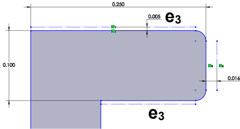
Figure 3.15 Offset the sides of the legs by e_3 inches to add flares for leg length less than 3/8 inches.
