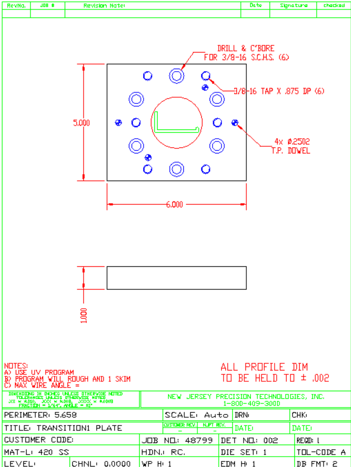
Figure C.2 Drawing sheet generated for Job 48799 depicting Transition 1 plate.
