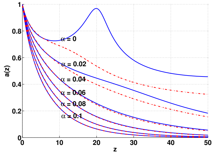
Figure 3.2 Effect of fiber loss on agreement between the PDE and ODE models. Dashed lines denote the PDE solution, and solids lines denote the ODE solution.
