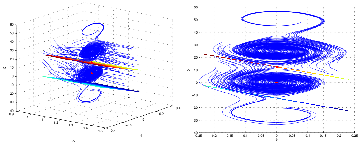
Figure 3.16 The blue curves are trajectories with random initial points. The red dots are fixed points of the system. The two tangent planes are spanned by two stable directions of two different saddle points.
