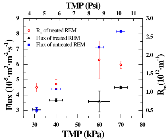
Figure 3.16 Flux and membrane resistance ( R_m ) under different TMPs in Psi and kPa in clean water test.
