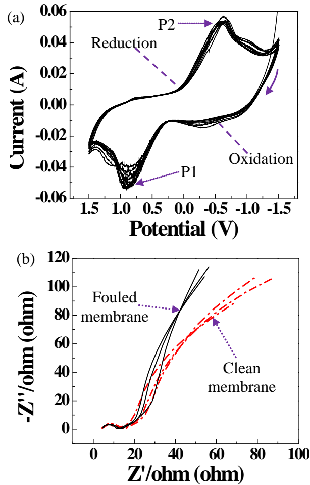
Figure 3.15 (a) I/V curves for REM filters in 0.5 M KCl solution when exposed to 20 mM K_3Fe(CN)_6^{3-} and (b) EIS spectra in complete frequency range for clean and fouled REM.
