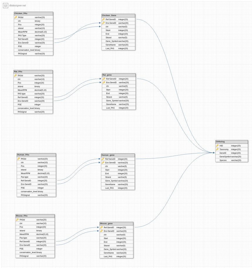
Figure 2.2 Relational Schema of PolyA_DB3. Shows the relationship between the relational tables of PolyA_DB3.
