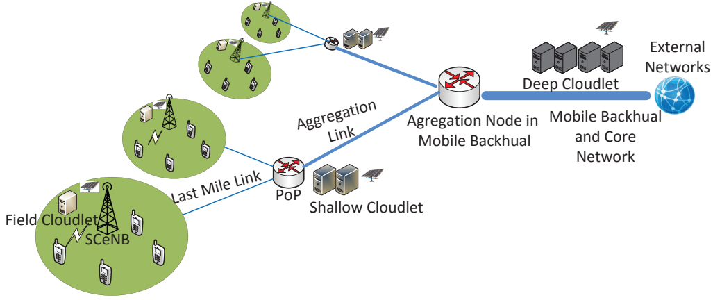
Figure 6.1 System model.
