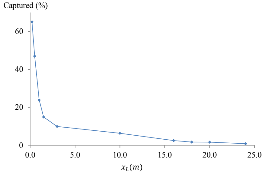
Figure B.5 The percentage of pollen rafts captured is shown as a function of x_L for u_w = 0.3 \text{ m/s} , y_d = 0.5 \text{ m} , a_p = 1 \text{ mm} , a_i = 2 \text{ mm} , and N = 3000 .
