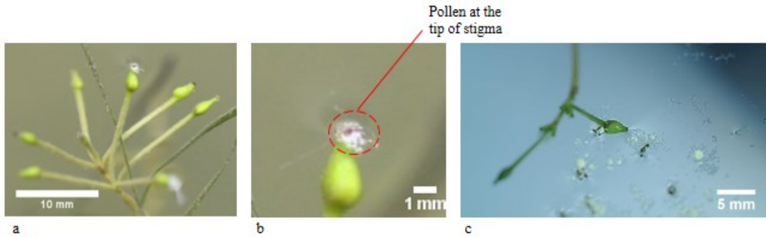
Figure 3.11 A female florescence at a water surface with two of its stigmas in contact with the water surface. (a) Female inflorescence, and (b-c) Magnified views of the stigmas in contact with the water surface. Notice the white colored pollen that is connected at their openings.
