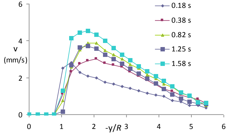
Figure 2.5 Temporal evolution of the streaming flow induced by the adsorption of a 2 mm particle. The velocity is shown at five different time intervals after the test particle came in contact with the water surface. The vertical component of velocity ( v ) is shown as a function of -y/R .
