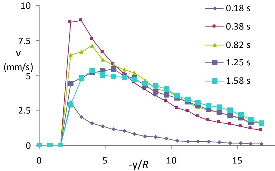
Figure 2.3 Temporal evolution of the streaming flow induced by the adsorption of a 650 \mu\text{m} particle. The fluid velocity is shown at five different time intervals after the test particle came in contact with the water surface. The vertical component of fluid velocity ( v ) is shown as a function of -y/R .
