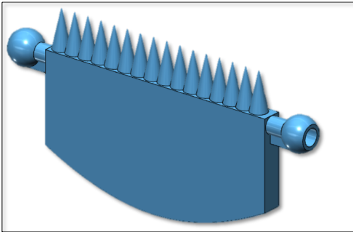
Figure 2.1 simplistic version of the lamellae and spinules used in the remora adhesive disk. Cone like structures were used to redesign the spinules. Ball like structure was used for the Ball and Socket structure. This ball structure is used to attaching the lamellae to the disk.
