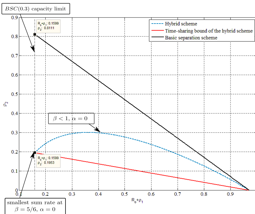
Figure 5.6 Combined rates R_o + \rho_1 vs. local randomness rate \rho_2 for p_{Y|X} = BSC(0.4) and P_{B|A} = BSC(0.3) .
