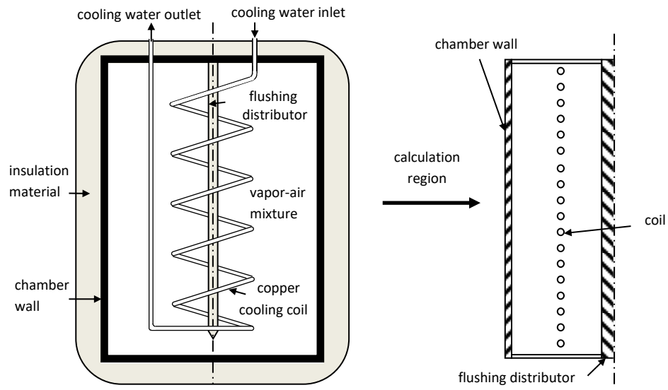
Figure 5.4-a Geometry simplification and simulation domain.
