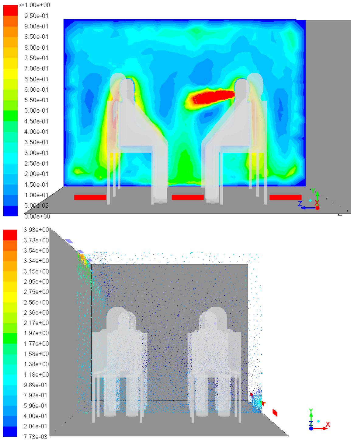
Figure 6.14 Results of CFD simulation for mean flow velocity at 0.5s.
