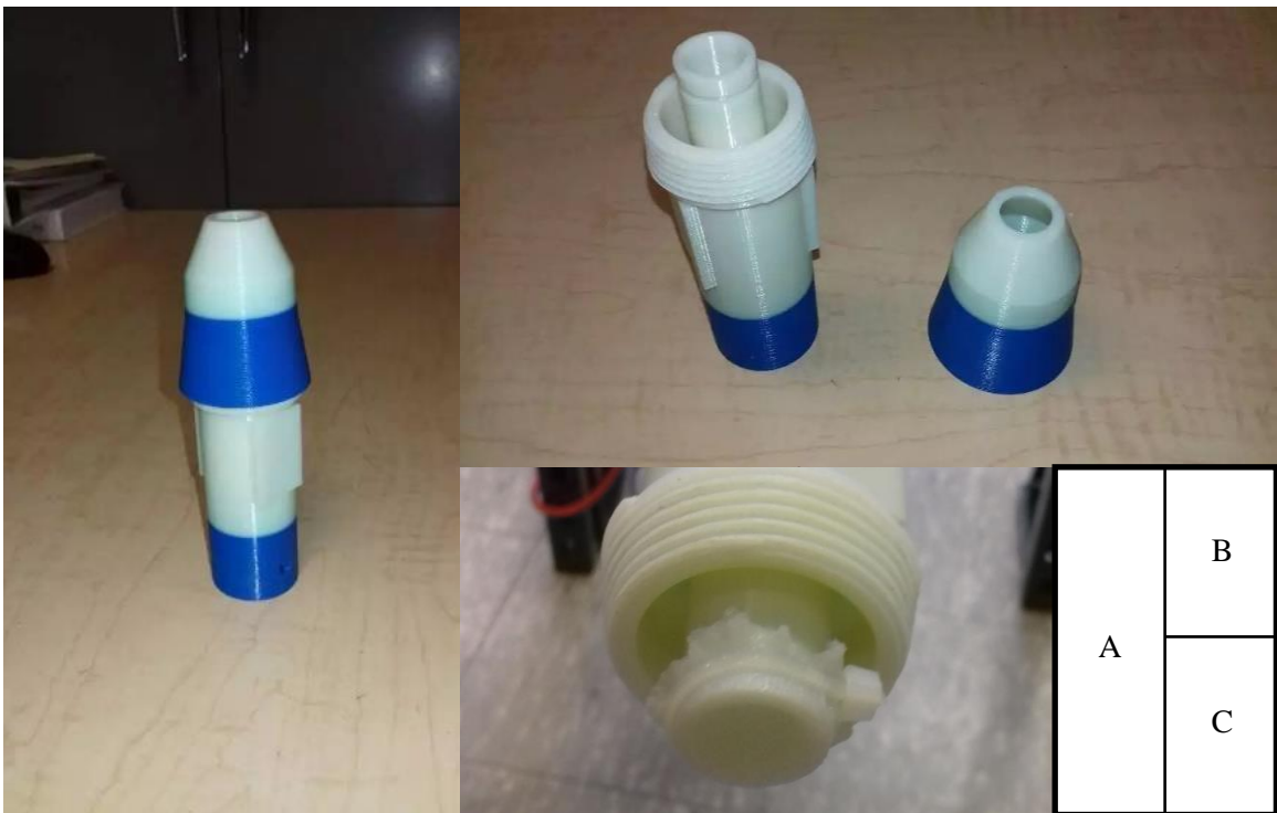
Figure 3.9 Receiver produced by 3-D printer.
