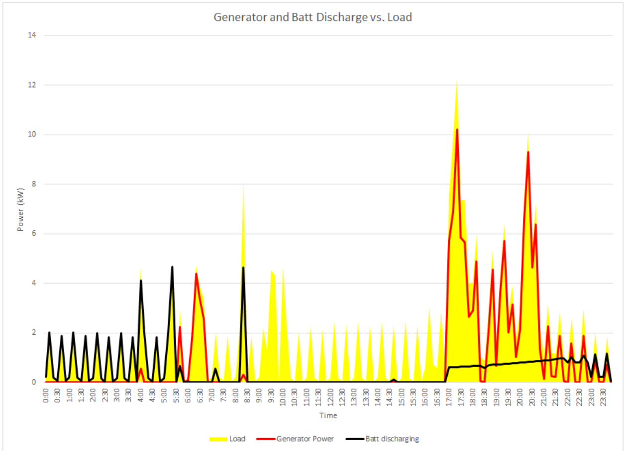
Figure 6.11 Generator and Batt Discharge vs. Time for simulation 9.
