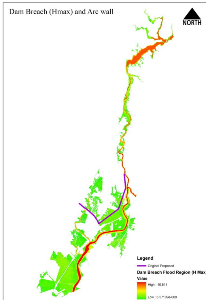
Figure 4.5 Dam Breach on Sunny Day (Hmax) and Arc Wall.
