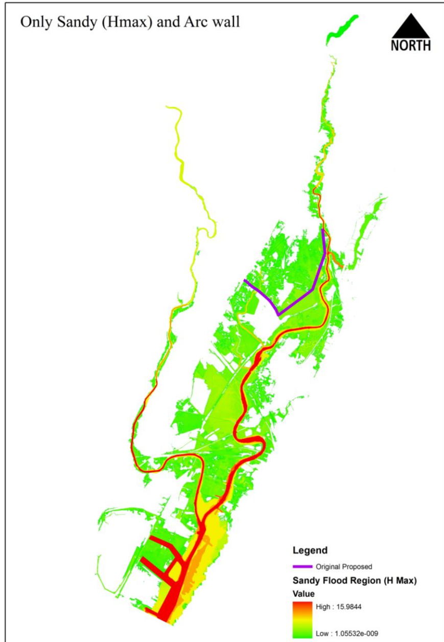
Figure 4.6 Only Super Storm and the Arc wall. Source: Base data considered from NJIT – FMERC Team. Data was edited for representation.
