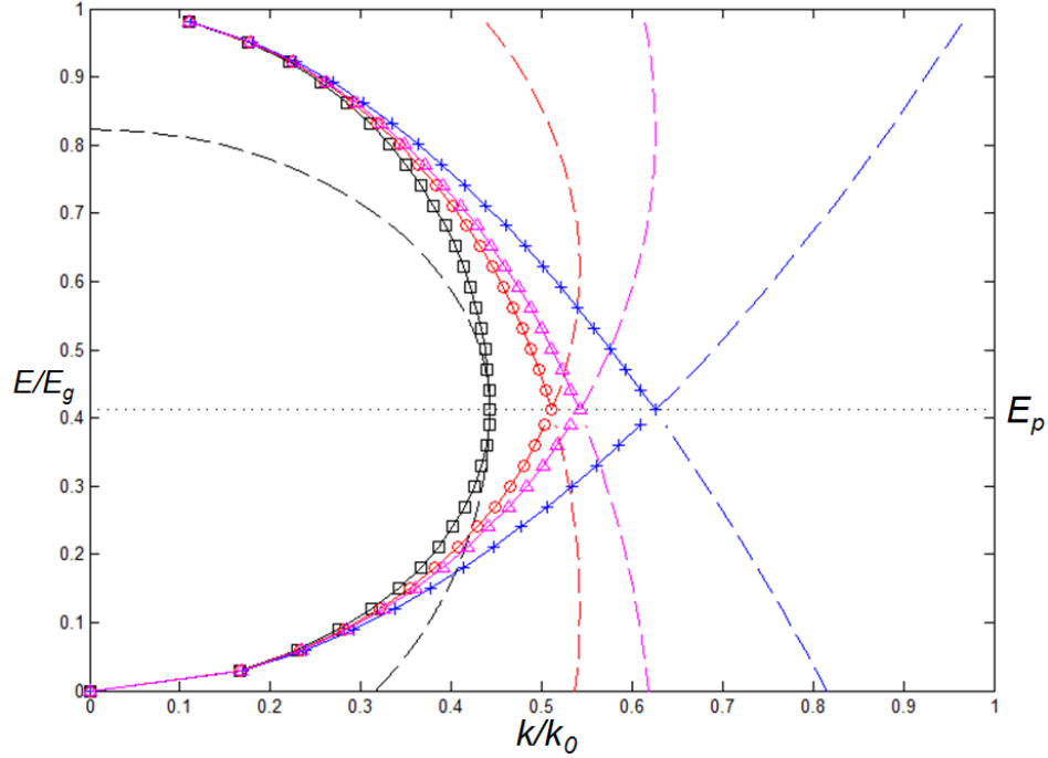
Figure 4.4 Energy vs imaginary wave vector within the band gap according to Eq. (4.10) and Eq. (4.11) and the tunneling path assumed in calculation (solid line) with various values of \beta . ( \square \beta = 2 , \circ \beta = 3 , \Delta \beta = 4 , + \beta \rightarrow \infty ). E_g is the energy band gap and E_p is the energy at which the tunneling carriers crossover from the hole branch to the electron branch while transversing through the energy band gap. Parameters used in the calculation: E_g = 1.52 \text{ eV} , m_c^* = 0.06m_0 , m_v^* = 0.09m_0 ; m_0 free electron mass, k_0 = \hbar^{-1}(2m_0)^{1/2} .
