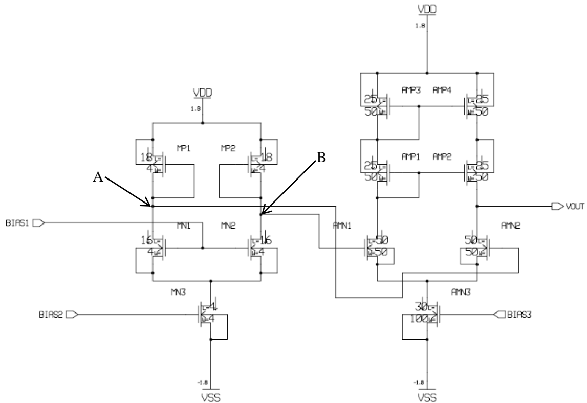
Figure 4.8 The equivalent circuit of the SD-MAGFET with the amplifier.
