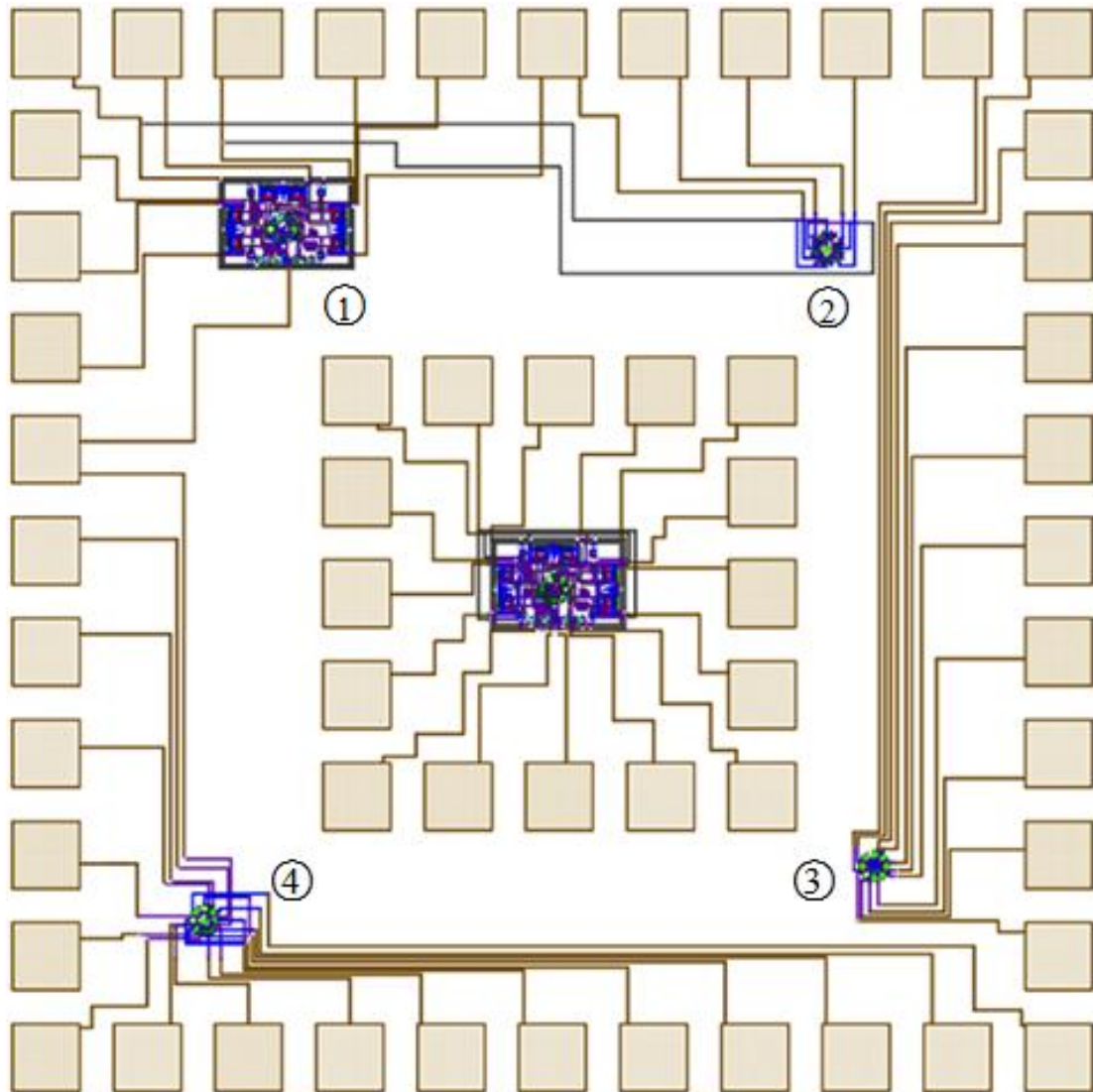
Figure 3.9 The chip layout of the three-dimensional MFS for further experiments.
