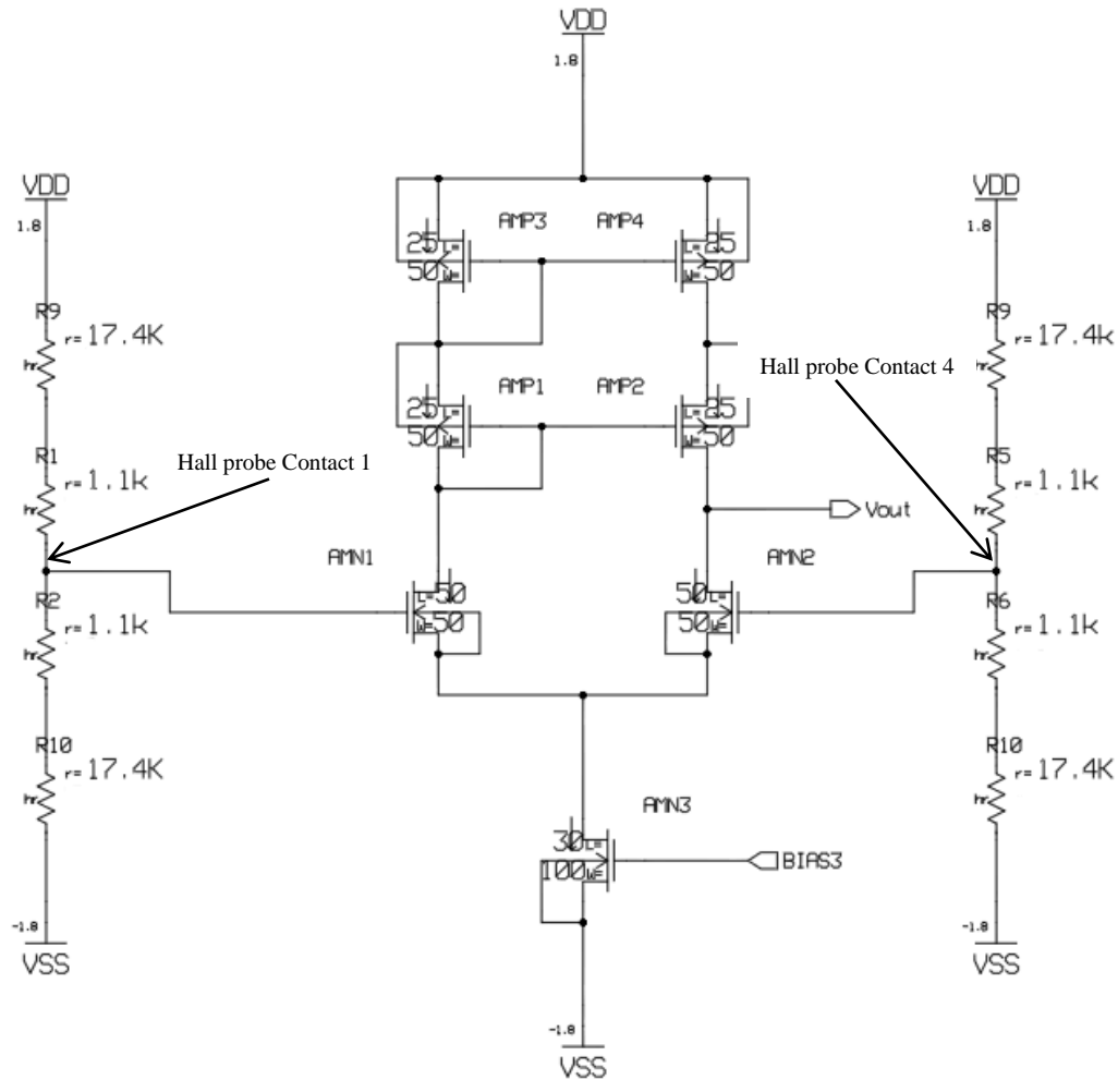
Figure 4.10 The equivalent circuit of the circular VHD connected with the amplifier.
