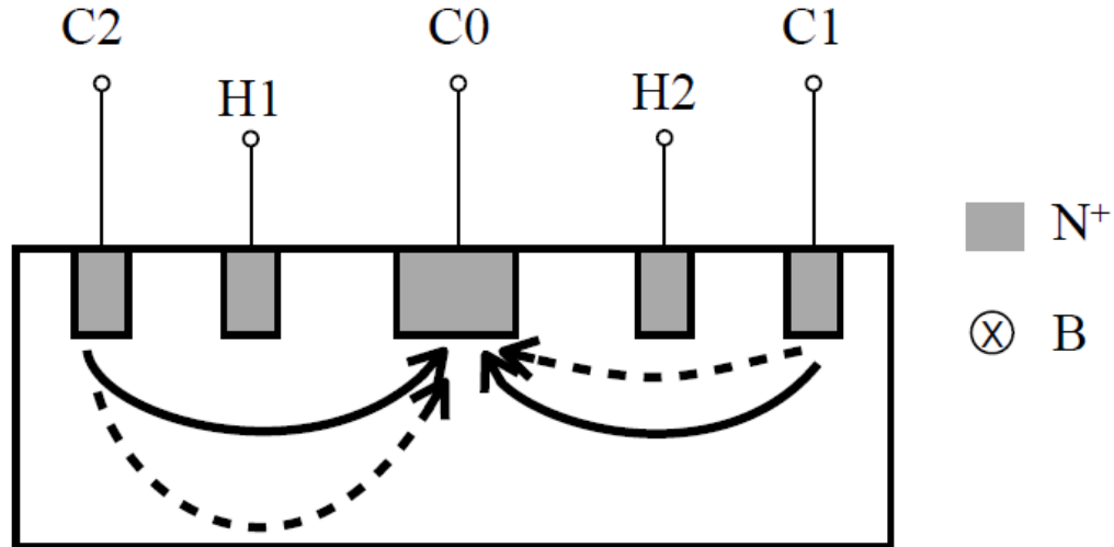
Figure 2.5 The vertical Hall Plate has three Power contacts and two Hall probe contacts. C1 and C2 are connected with VDD, and C0 is connected with GND. Current will flow from C1 and C2 to C0. H1 and H2 are used to detect the variation of current caused by the magnetic field.
