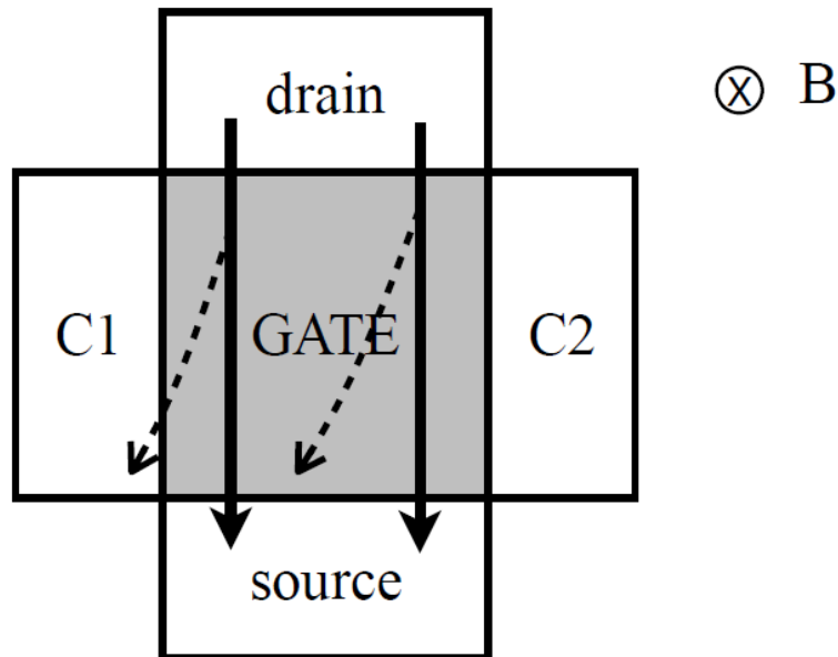
Figure 2.3 The top view of the horizontal MFS in the MOS structure adapted from [4].
