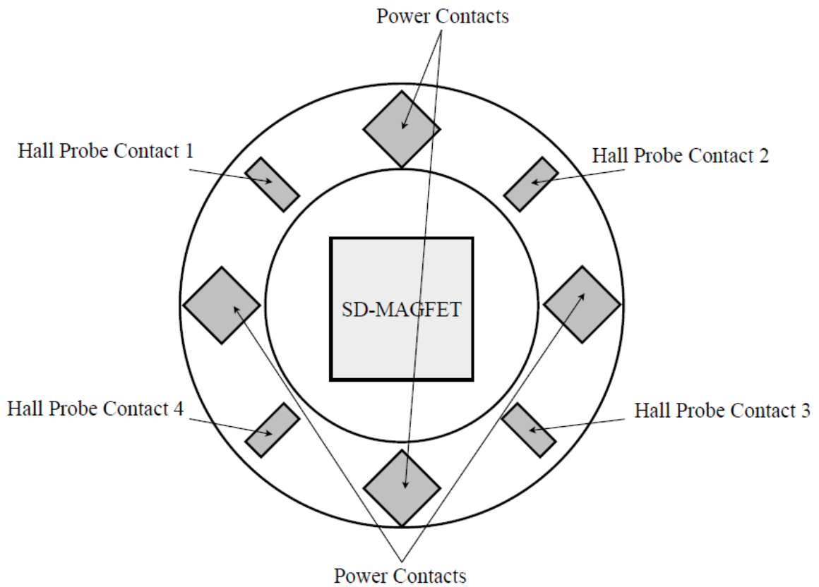
Figure 3.6 The entire pattern of the three-dimensional MFS is shown in this figure. The SD-MEGFET which has the independent power supply is located at the center of the device. The detail of the circular VHD located around the SD-MAGFET is also shown in this figure.
