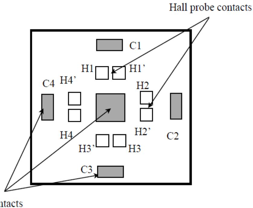
Figure 2.9 The three-dimensional MFS with split Hall probe contacts adapted from [9].
