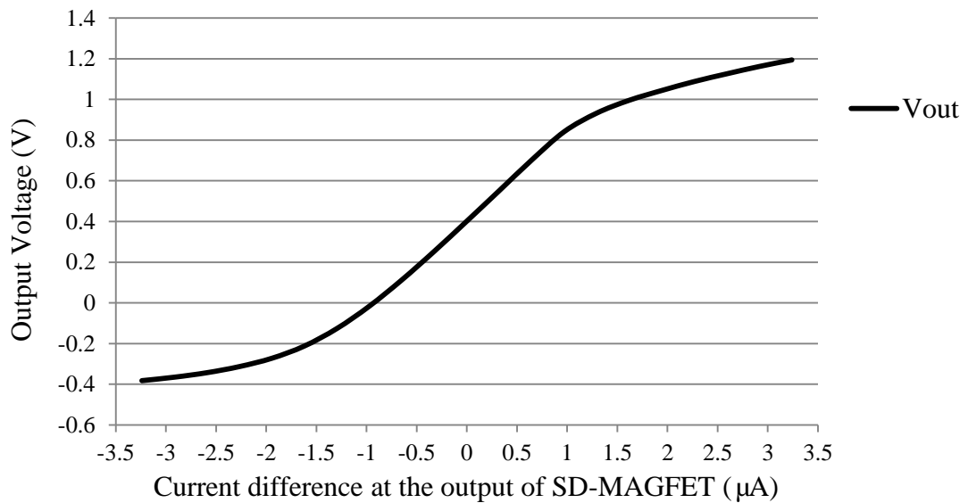
Figure 4.9 The voltage characteristic of the amplifier at the output node.
