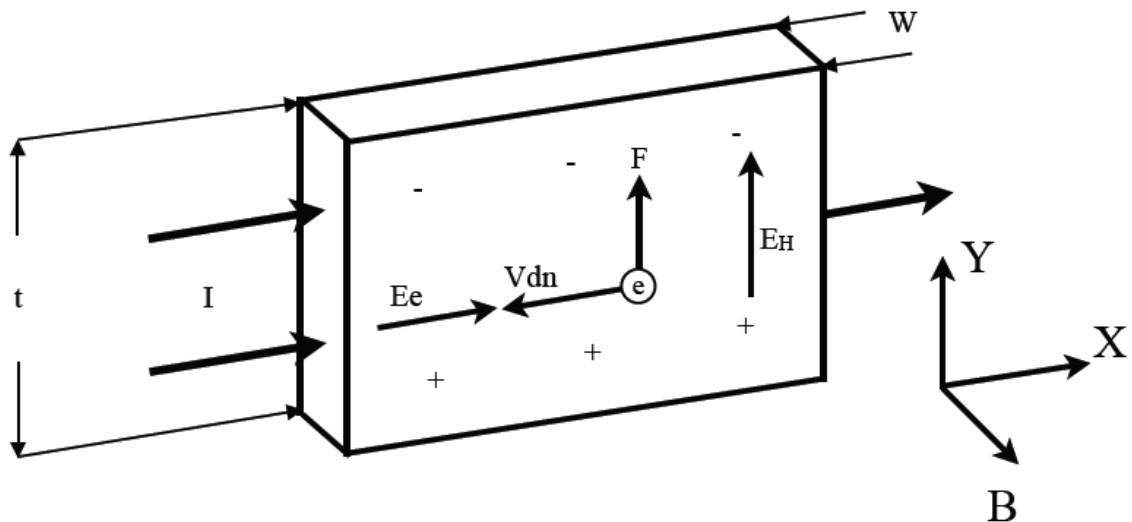
Figure 2.1 A Hall Plate which suggests the Hall Effect.
