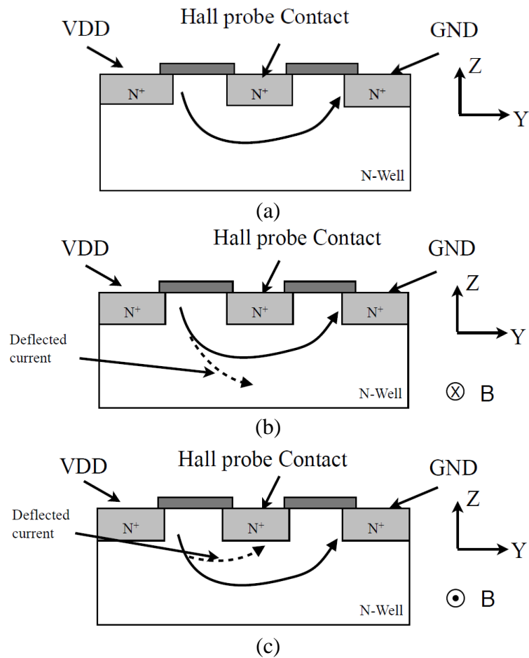
Figure 3.4 Current flowing in the circular VHD with or without the magnetic field. Figure 3.4(a) shows the current-flow in the circular VHD. Figure 3.4(b) and (c) reflect deflected current with the external magnetic field.
