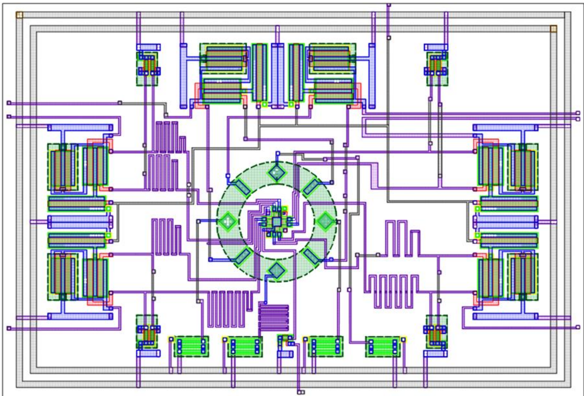
Figure 3.8 The entire layout of the three-dimensional MFS.
