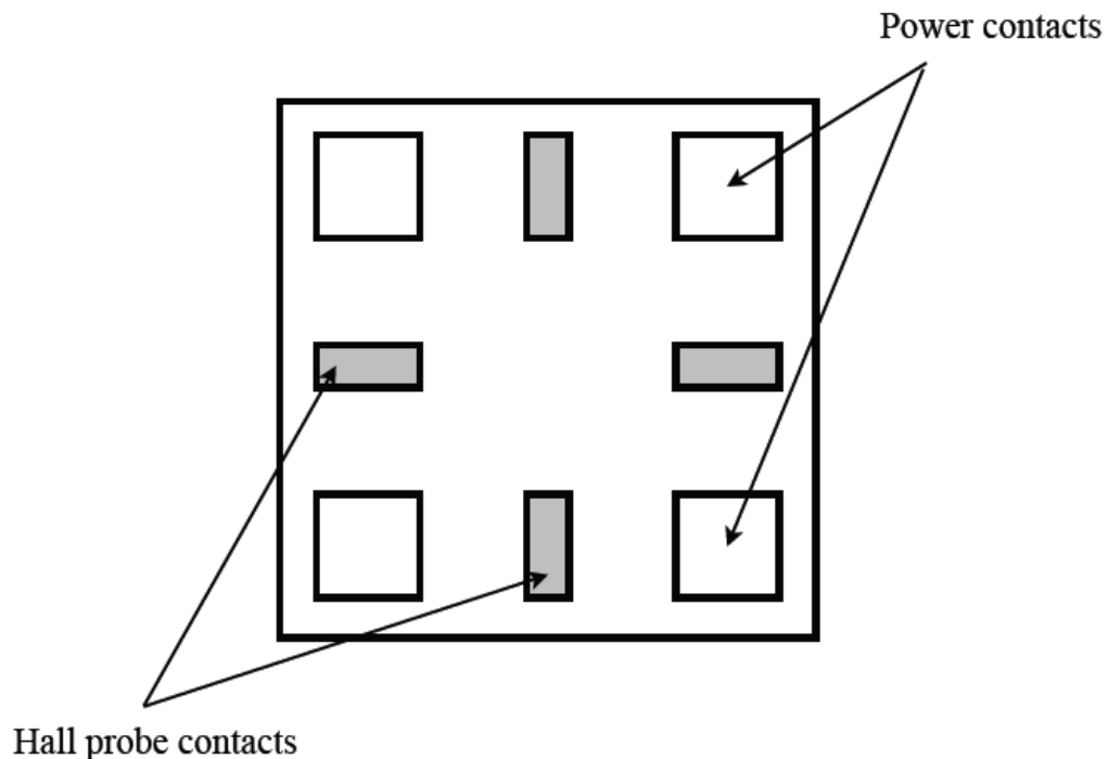
Figure 2.10 The Square-shaped three-dimensional MFS with power supply contacts located at the corner adapted from [10].
