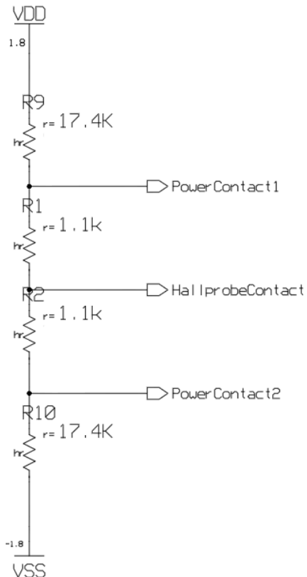
Figure 4.5 The equivalent circuit of the circular VHD.
