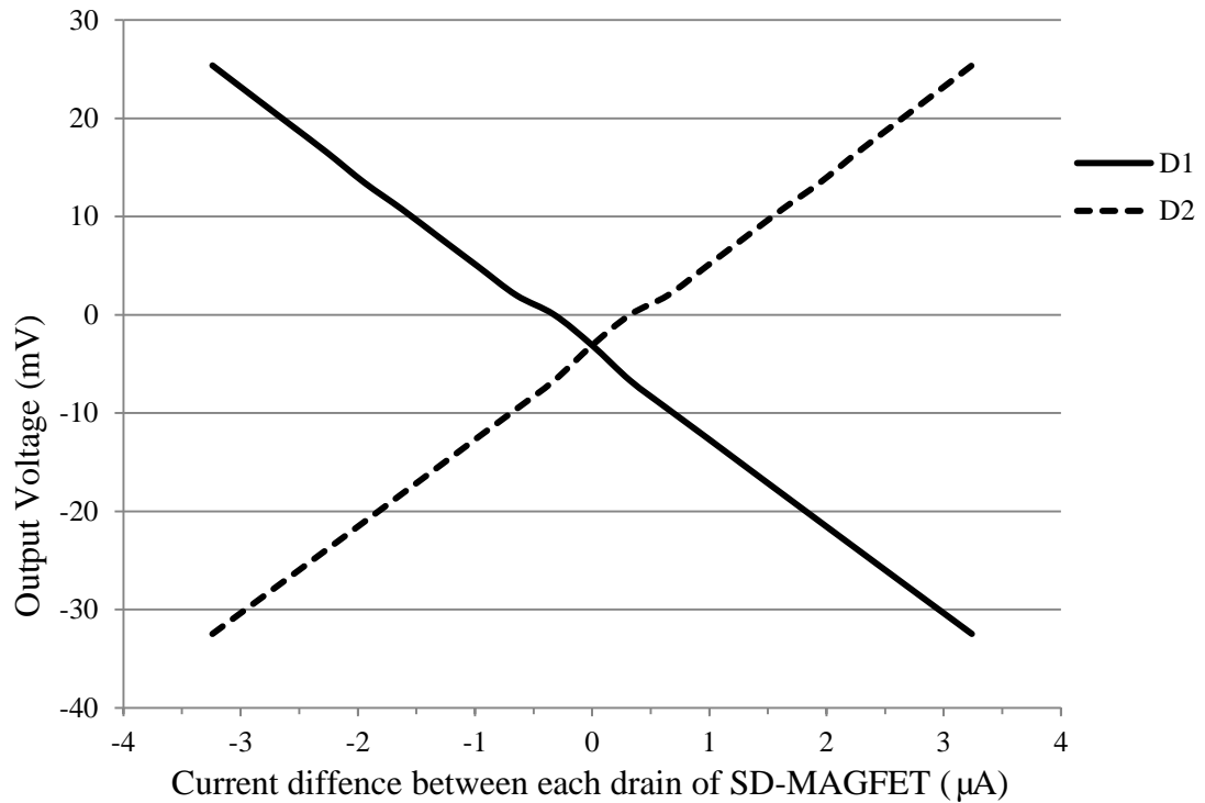
Figure 4.3 The output voltage swing of the SD-MAGFET.
