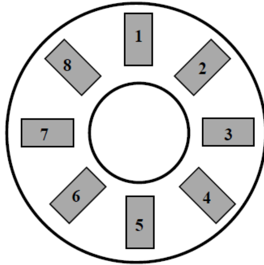
Figure 2.8 The circular-shaped two-dimensional MFS with a Phase Sampling system adapted from [8].
