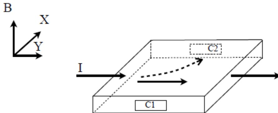
Figure 2.2 A conventional Hall Plate which shows the current flow direction (solid line) and deflected current (dash line) by external magnetic field.
