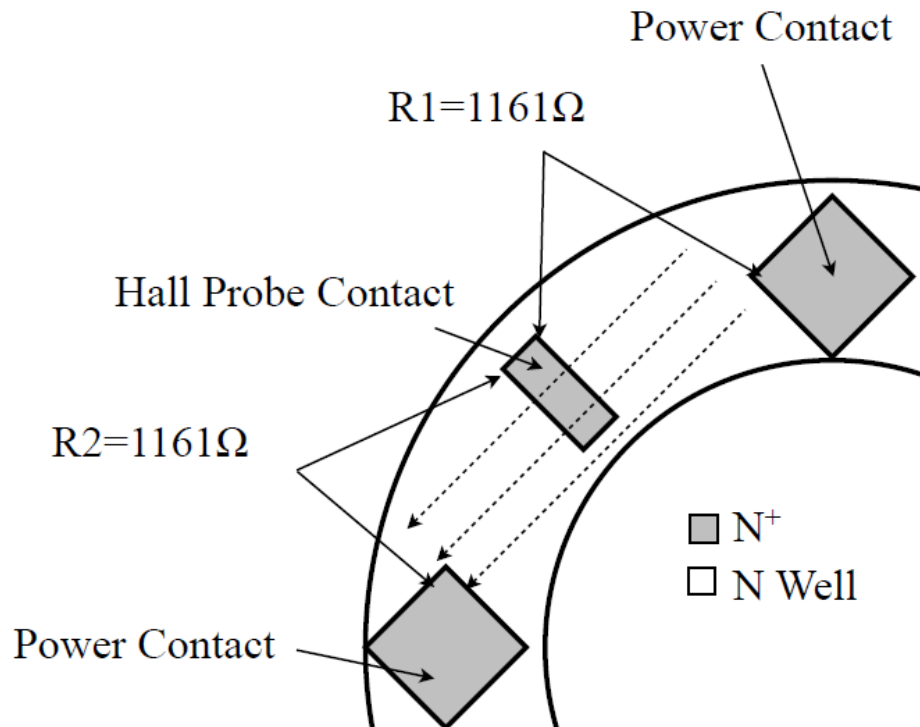
Figure 3.5 One fourth of the circular Hall device. From the extraction, resistance between each power contact and Hall probe contact is designed as 1161 ohms.
