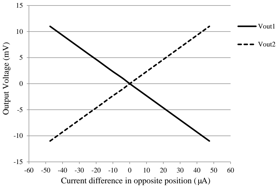
Figure 4.6 The output voltage swing after applying the horizontal magnetic field.
