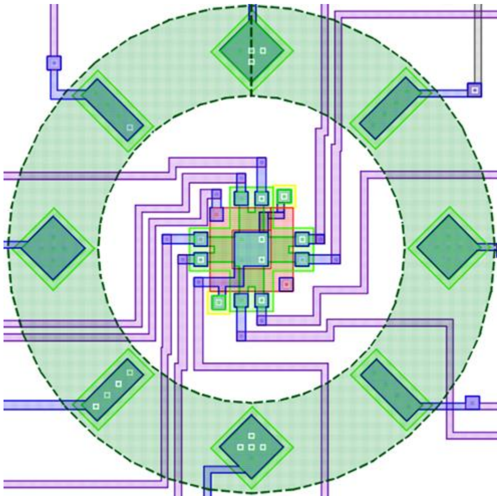
Figure 3.7 The layout of the circular VHD for the horizontal magnetic field detection.
