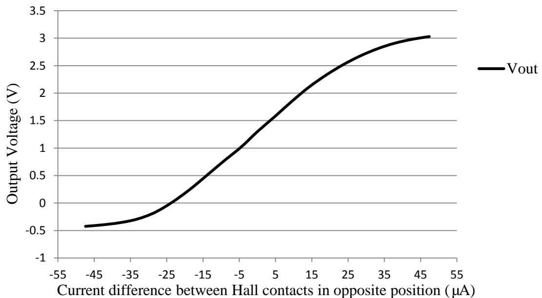
Figure 4.11 The simulation result of the circular VHD connected with the amplifier.
