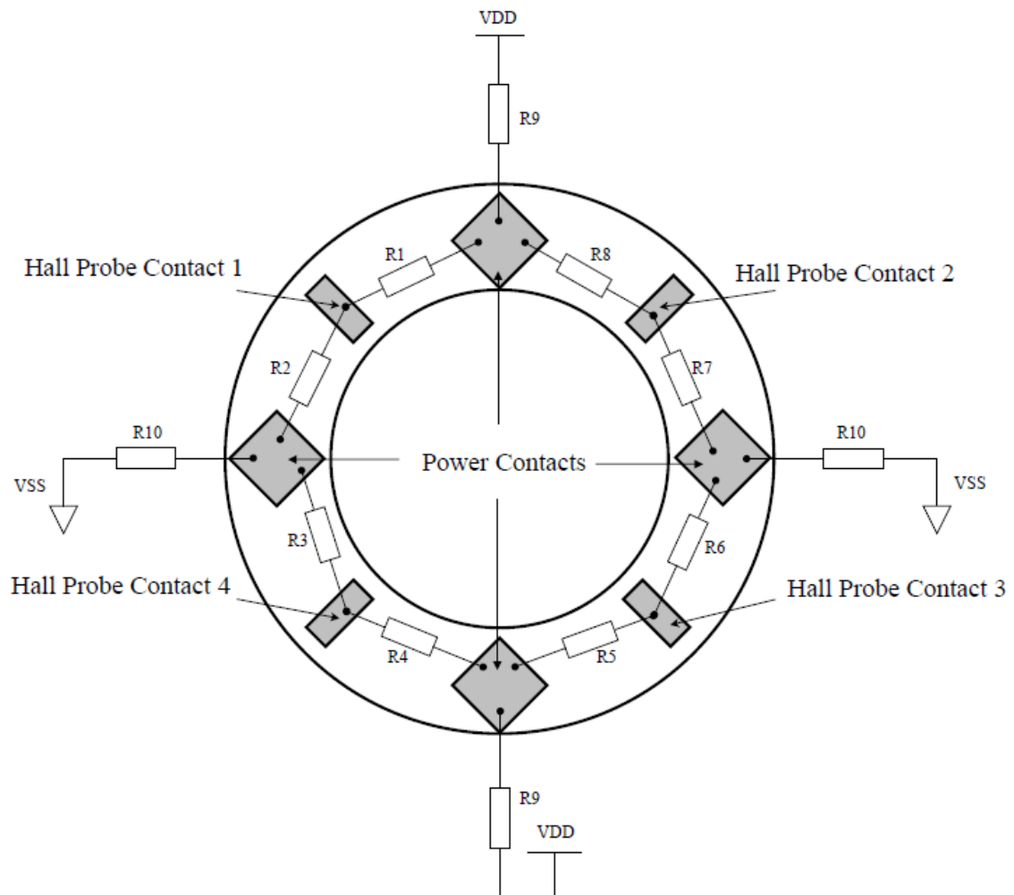
Figure 4.4 The conversion of the VHD in the form of resistor.
