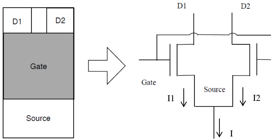
Figure 4.1 The equivalent circuit of the SD-MAGFET.
