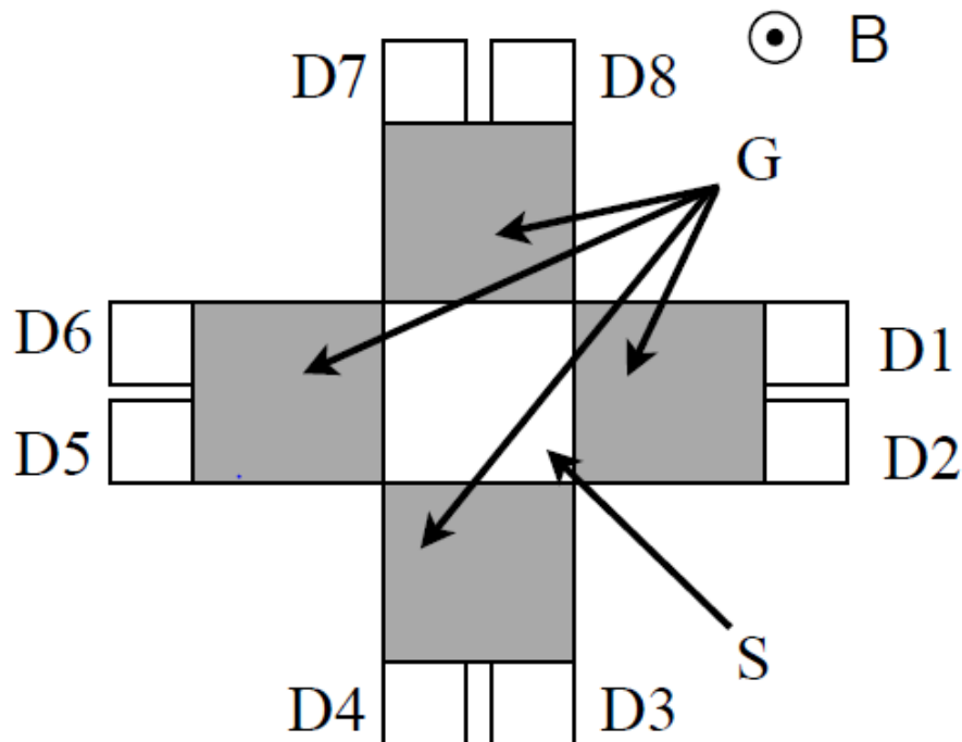
Figure 3.2 Four SD-MAGFETs with a common source connection.
