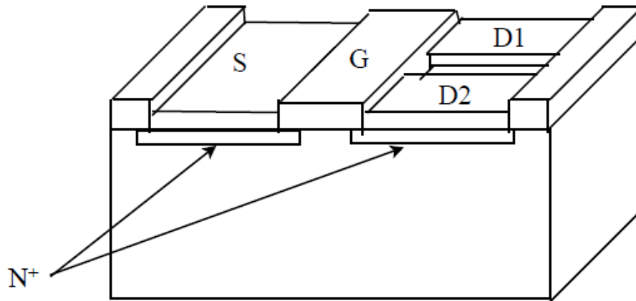
Figure 2.4 The three-dimensional view of the SD-MAGFET adapted from [5].
