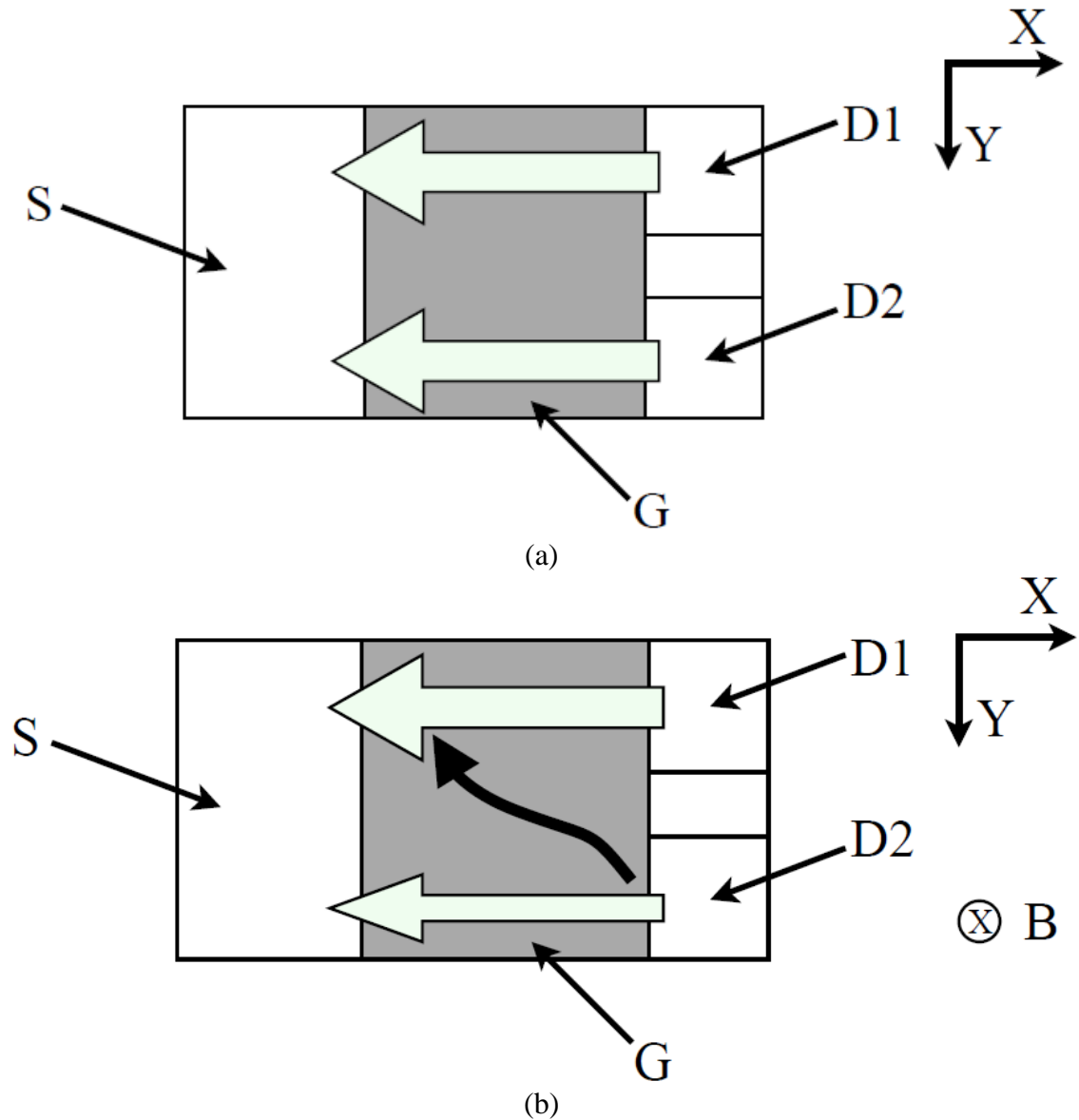
Figure 3.1 Current flows in SD-MAGFET with or without the magnetic field. Figure (a) demonstrates the current-flow without the external magnetic field, and Figure (b) reflects the variation of current inside the SD-MAGFET with the vertical magnetic field.
