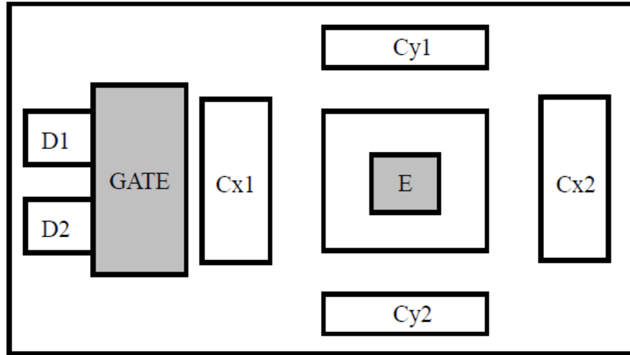
Figure 2.11 The three-dimensional MFS in BiCMOS technology adapted from [11].
