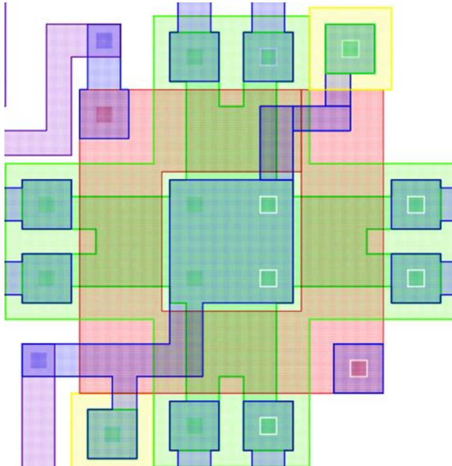
Figure 3.3 The entire layout design for the vertical magnetic field detection
