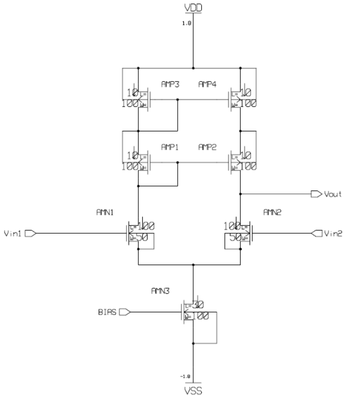
Figure 4.7 The equivalent circuit of the cascode amplifier.
