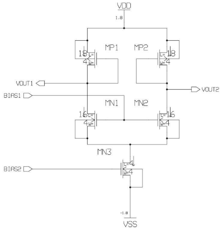
Figure 4.2 The equivalent circuit of the SD-MAGFET. Circuit of the pMOS active load and the current sink is shown in this figure as well. The SD-MAGFET is split into two nMOSs.
