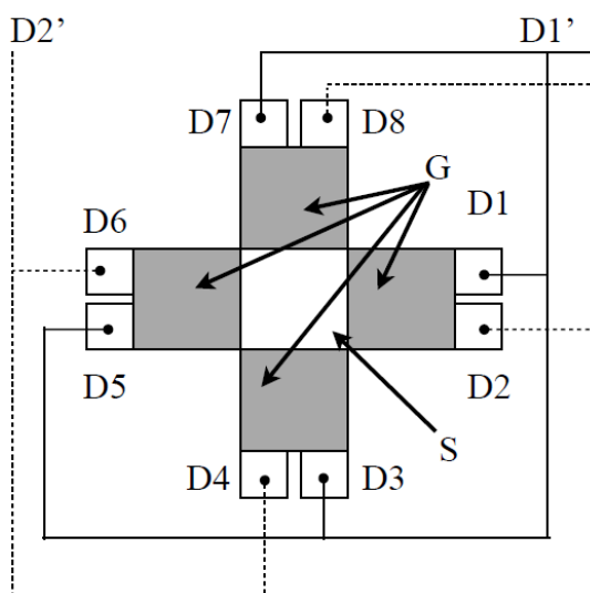
Figure 5.1 Four right side drains and four left side drains are connected separately to increase the performance of the SD-MAGFET.
