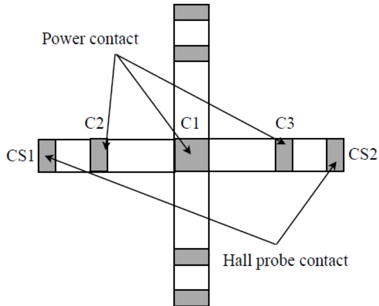
Figure 2.7 The bar-shaped two-dimensional MFS adapted from [7].
