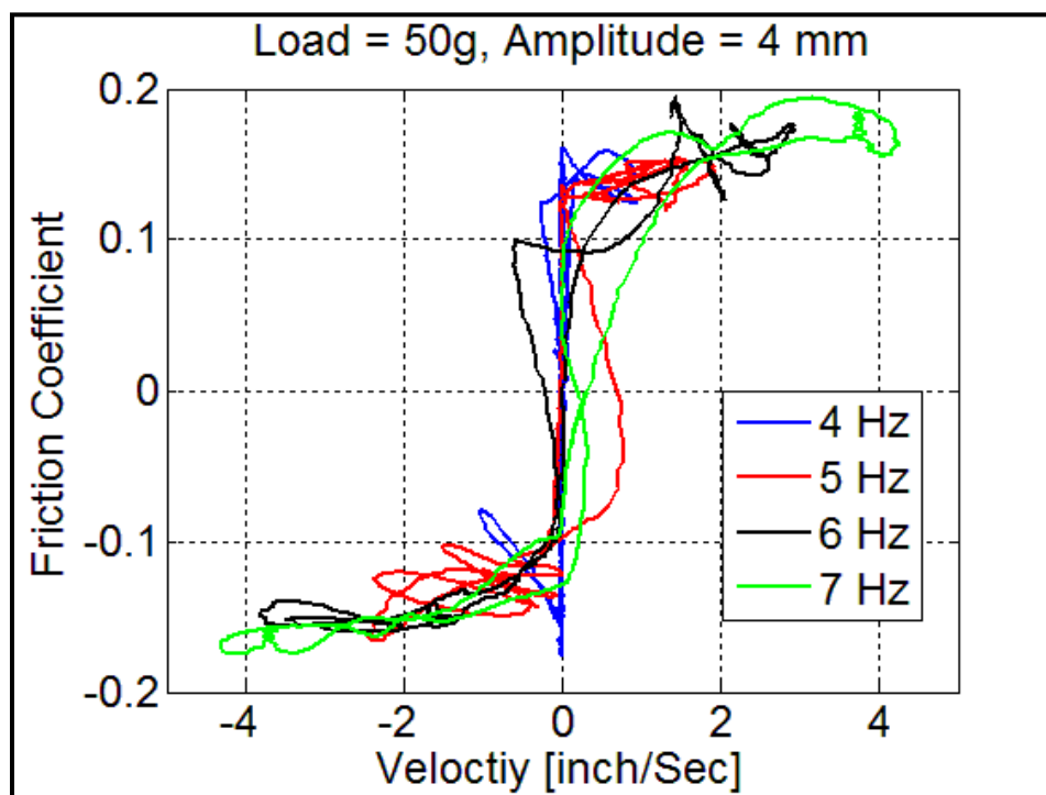
Figure 3.38 Teflon – Teflon with a 50g load, amplitude = 4 mm and different frequencies.
