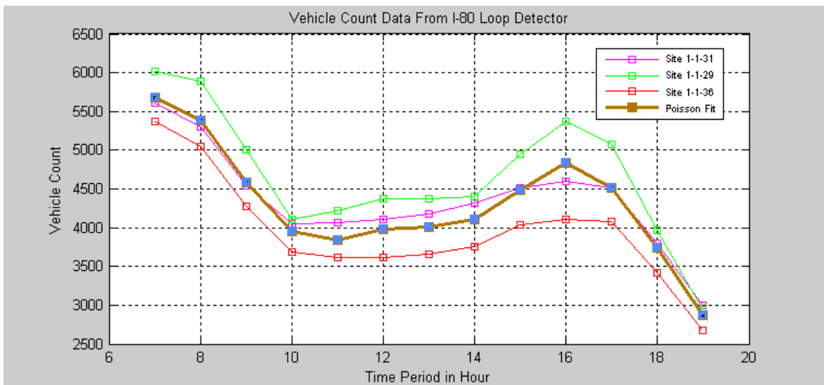
Figure 4.3 Poisson Fit of vehicle count data
