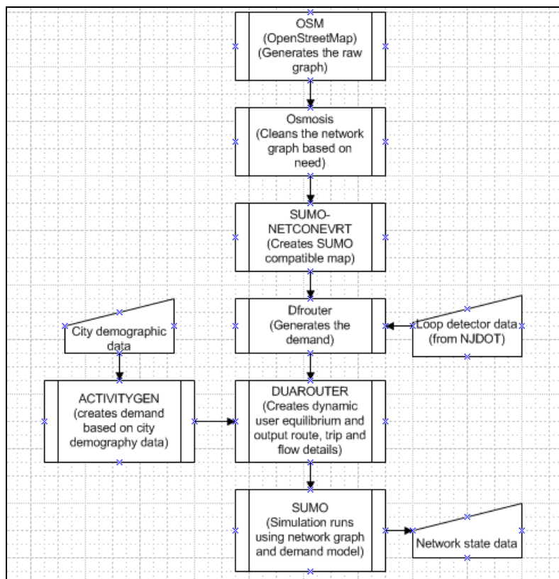
Figure 6.2 A schematic diagram of simulation experiment steps
