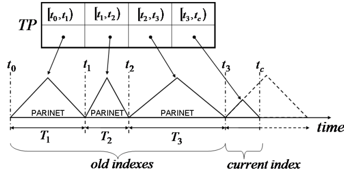
Figure 3.2 Example of a T-PARINET Index Structure
