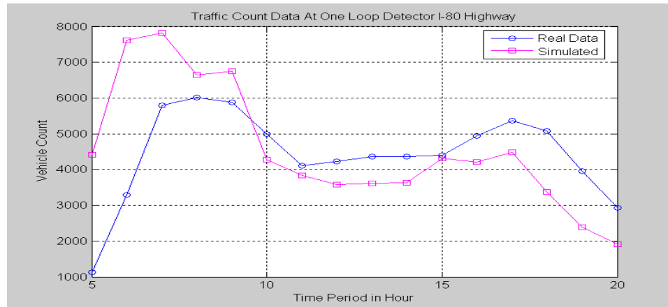
Figure 7.3 Prediction using simulated data
