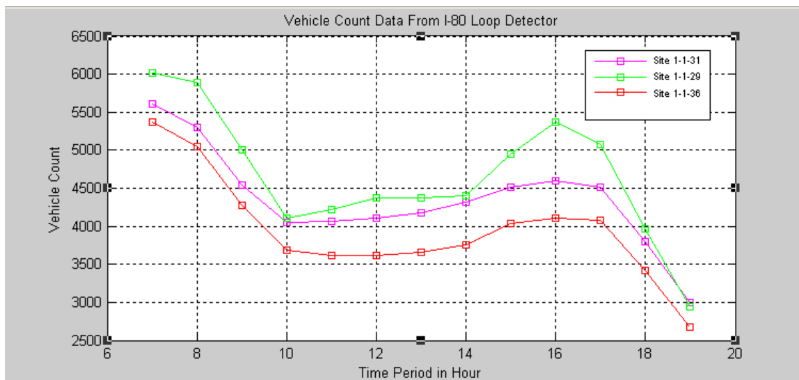
Figure 4.2 Vehicle count data at three sites on I-80
