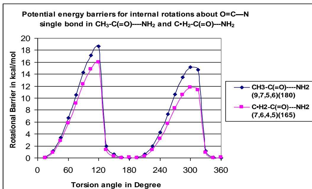
Figure 1.3.2 Potential energy barriers for internal rotations about O=C—N single bond in \text{CH}_3\text{-C(=O)}\text{---NH}_2 and \text{C}\cdot\text{H}_2\text{-C(=O)}\text{---NH}_2
