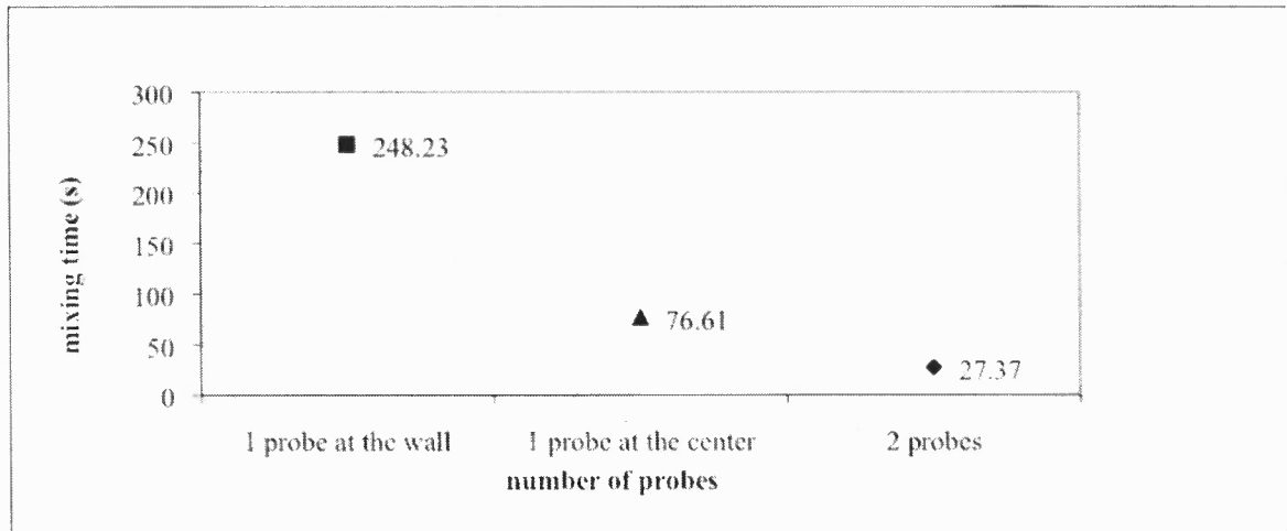
Figure 4.4 Experimental mixing time for different number and positions of the conductivity probes in the tank using the conductivity method (unbaffled condition; 100 rpm). When two probes were in place the mixing time in the figure refers to that measured near the wall.
