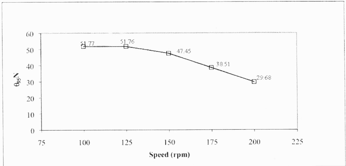
Figure 3.15 Plot of \theta_{95N} as a function of agitation speed under partially baffled conditions.
