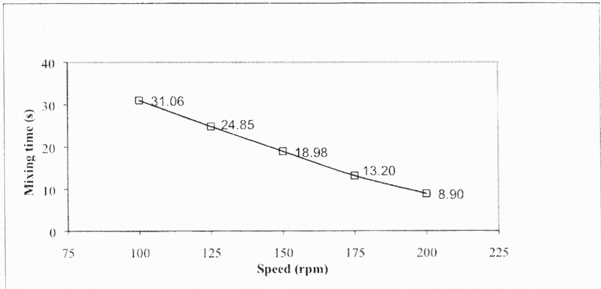
Figure 3.14 Plot of mixing time as a function of agitation speed under partially baffled conditions.
