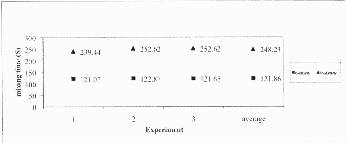
Figure 4.1 Comparison of three experiments in which the mixing time was obtained by the conductivity method and colorimetric method in the presence of one probe located at the wall.
