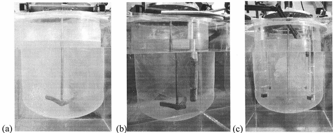
Figure 2.1 Mixing system used in this work: (a) un baffled tank (b) partially baffled tank with beavertail baffle (c) fully baffled tank
