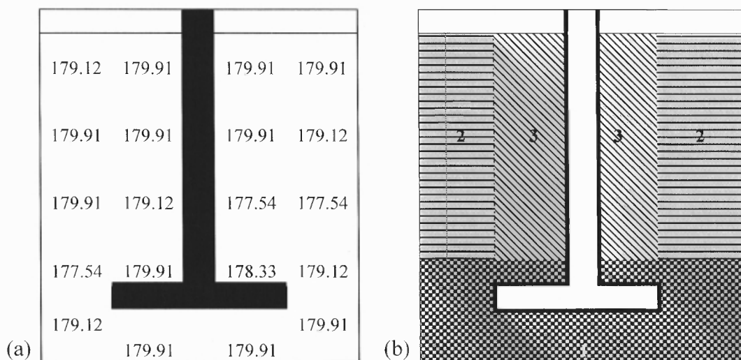
Figure 3.7 (a) Individual mixing times obtained with the colorimetric method in absence of conductivity probe (b) sequence in which regions changed color in absence of conductivity probe System: un baffled tank; Agitation speed= 100 rpm.
