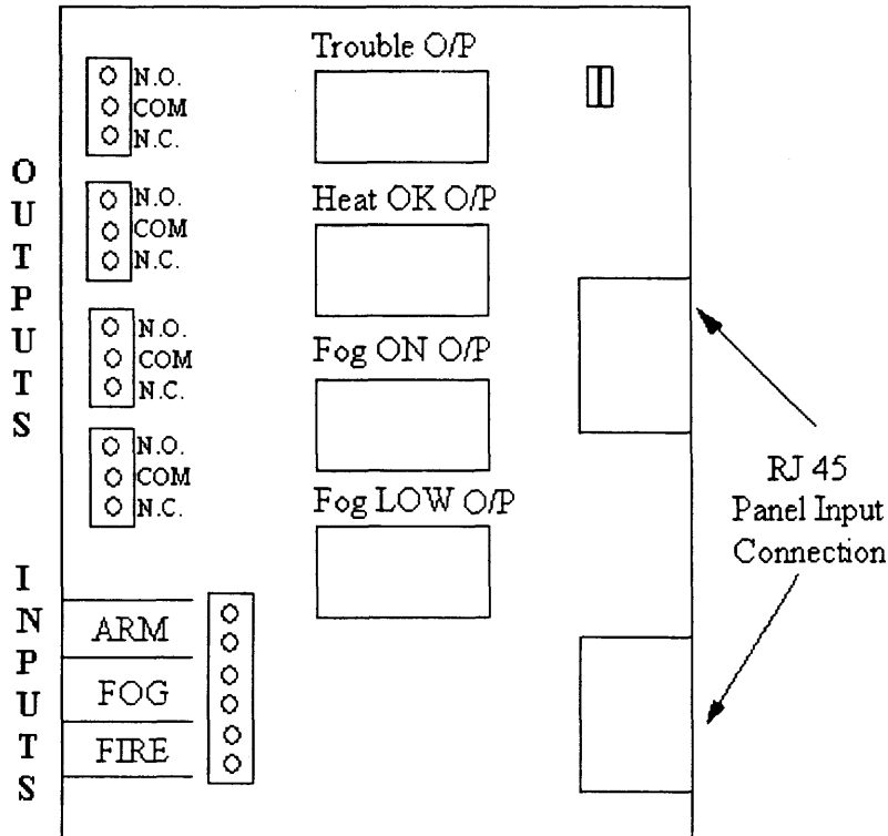
Figure 2.9 Panel Input/Output Board
