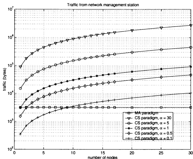
Figure 3.1 Traffic generated around the management station
