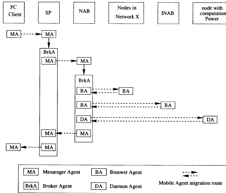
Figure 2.3 Agents used to implement routing algorithms based on GA
