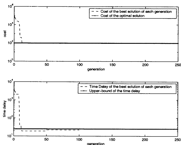
Figure 2.10 GA is stopped after getting optimal solution
