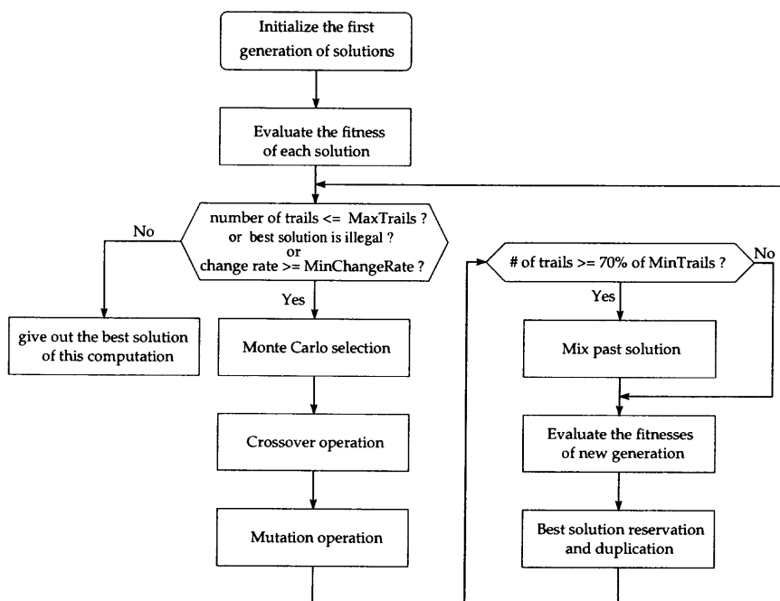
Figure 2.2 Flow chart of GA
