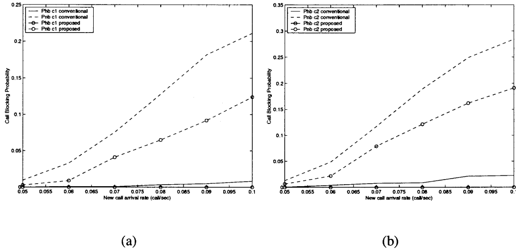
Figure 4.6 Call blocking probabilities under test traffic scenario 2. (a) Call blocking probabilities for class 1 users. (b) Call blocking probabilities for class 2 users.
