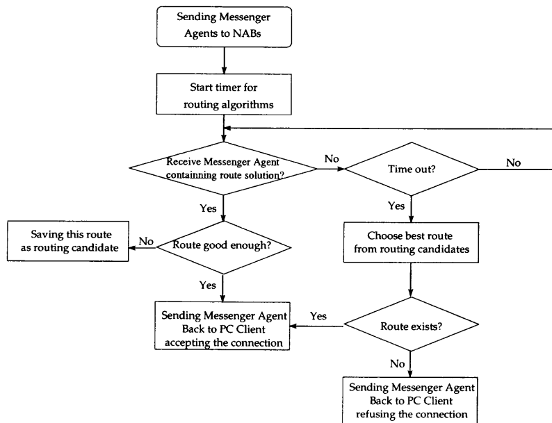
Figure 2.4 Algorithm for Broker Agent in SP to choose a route for its client
