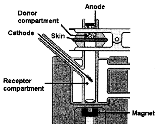
Figure 1.2 Diagram of a Franz cell apparatus for iontophoretic delivery. The drug and its vehicle are loaded into the donor compartment. The drug diffuses through the skin and into the receptor compartment. In the iontophoretic system shown here, the anode is placed at the donor cell and the cathode at the receptor cell.
