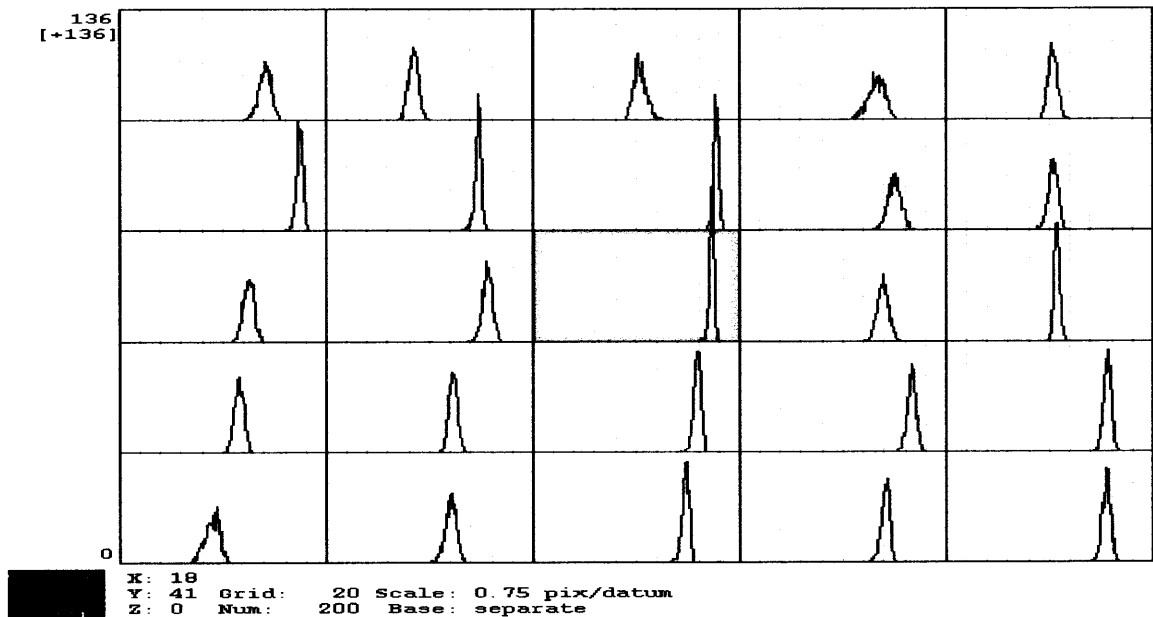
Figure 6.10 (b) Represents the histogram of the correlation coefficient values ranging from -1 to +1 obtained using the block bootstrap resampling technique for the voxels shown in Figure 6.8.
