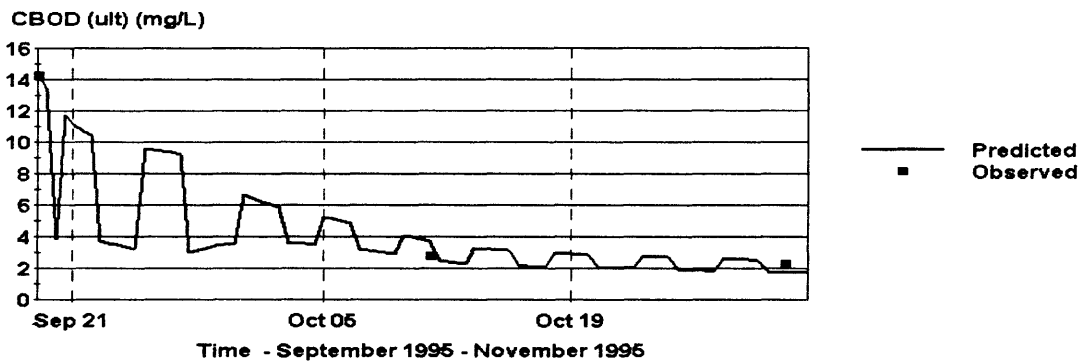
Figure 5.15(b) BOD Validation – Segment 7 (Temporal Variation).
