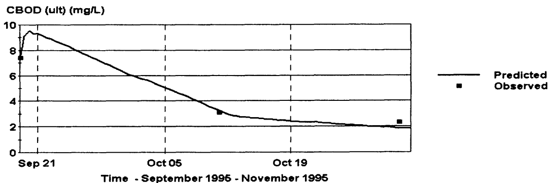
Figure 5.15(a) BOD Validation – Segment 4 (Temporal Variation).
