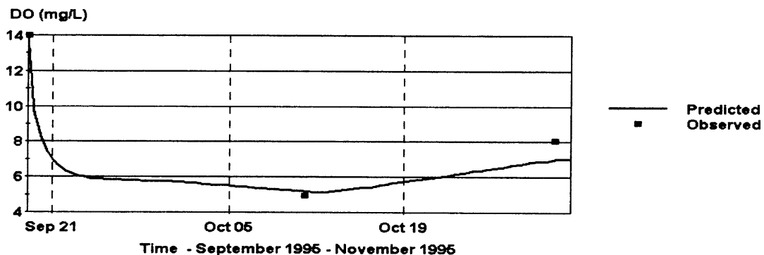
Figure 5.13(e) DO Validation – Segment 15 (Temporal Variation).
