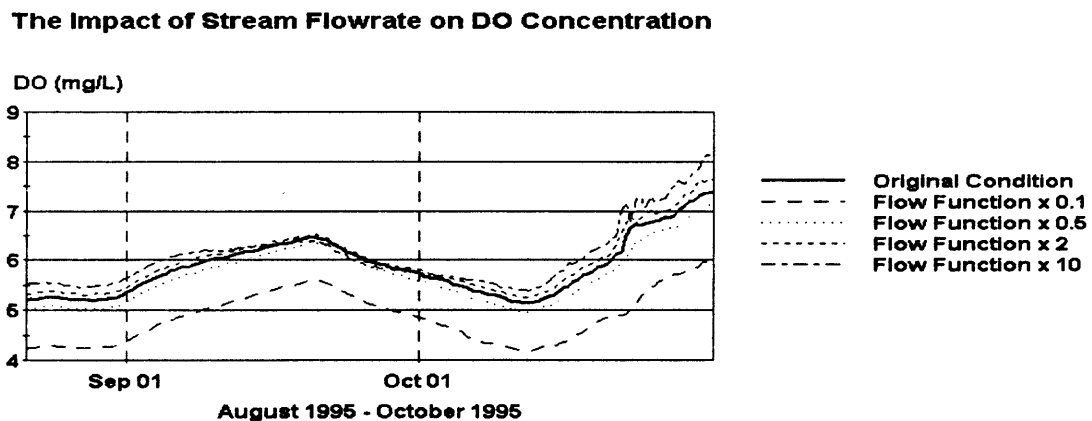
Figure 6.12 The Impact of Stream Flowrate on DO Concentration.
