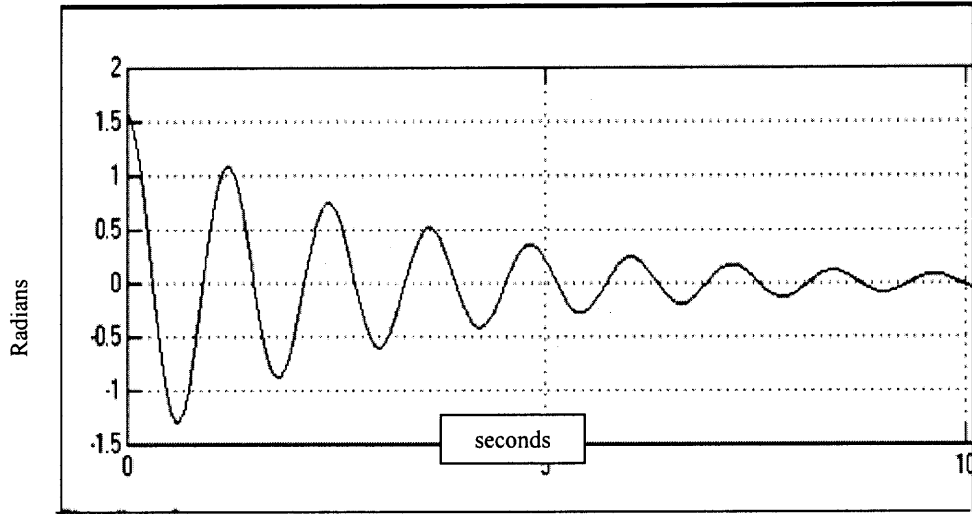
Figure 4.62. Normal Simulation
