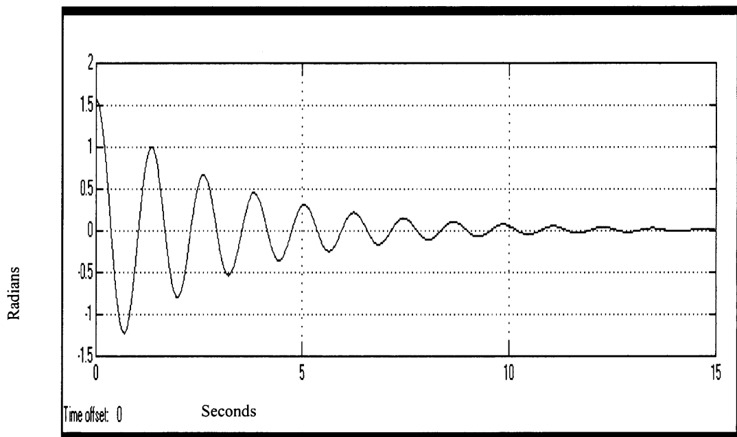
Figure 3.5. Underdamped Oscillator-Position-Second Order Differential Equation (muscle contribution-switch OFF)
