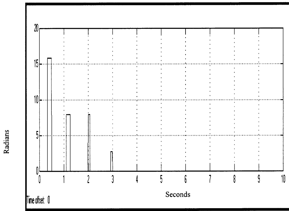
Figure 3.23. Switch On/Off (Switch On)- Muscle Torque –
