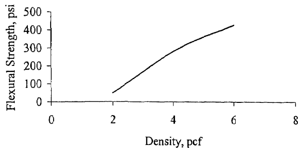
Figure 8: Flexural strength verses density of PVC foams illustrates the directly proportional relationship.
