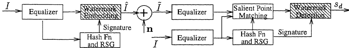
Figure 7.2 Watermark embedding and detection protocol
