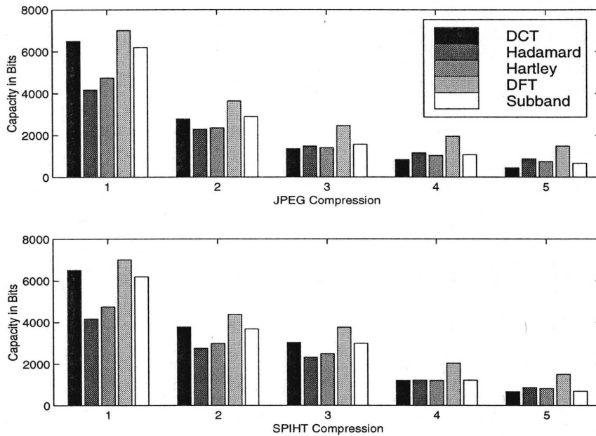
Figure 3.7 Average capacity estimates for 15 256 \times 256 images. The indices for JPEG compression correspond to different JPEG quality factors. (1 - lossless compression, 2 - 75%, 3 - 50%, 4 - 35%, 5 - 25%) The indices for SPIHT compression correspond to different bit rates (1 - lossless, 2 - 1 bpp, 3 - 0.75 bpp, 4 - 0.5 bpp, 5 - 0.35 bpp).
