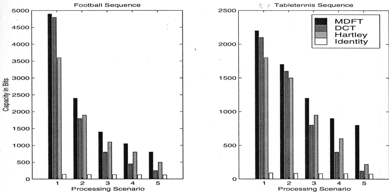
Figure 3.10 Channel capacities of different decompositions for Football and Tabletennis Sequences. The processing scenarios 1-5 correspond to lossless compression, and compression ratios of 10, 25, 50 and 100 (MPEG-2) respectively.
