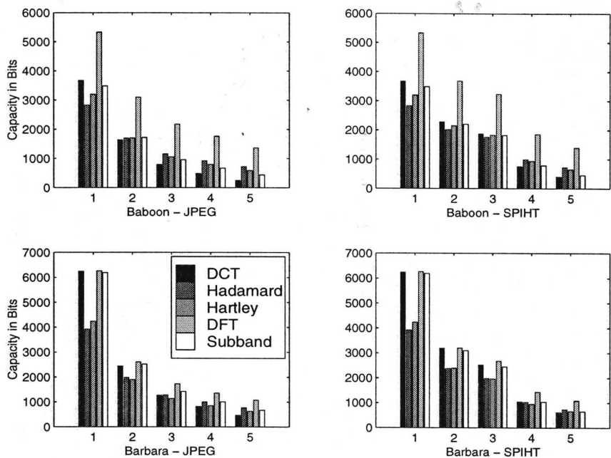
Figure 3.8 Capacity estimates for 256 × 256 Baboon and Barbara images. The indices for JPEG compression correspond to different JPEG quality factors. (1 - lossless compression, 2 - 75%, 3 - 50%, 4 - 35%, 5 - 25%) The indices for SPIHT compression correspond to different bit rates (1 - lossless , 2 - 1 bpp, 3 - 0.75 bpp, 4 - 0.5 bpp, 5 - 0.35 bpp).
