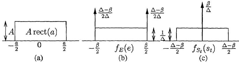
Figure 4.9 (a) The rectangular function. (b) and (c) Probability distributions of f_E(e) - distortion introduced by the modified embedding function, and f_{S_t}(s_t) - noise introduced due to modified embedding function.
