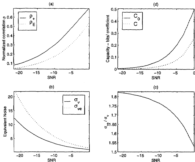
Figure 4.12 Performance of optimal CP-SNS. (a) Plot of normalized correlation vs. SNR for non oblivious ( \rho_+ ) and optimal CP-SNS ( \rho_E ). (b) Equivalent noise for optimal CP-SNS ( \sigma_{ve} ) and non oblivious method ( \sigma_v ). (c) The ratio \frac{\sigma_{ve}}{\sigma_v} . (d) Achievable capacity in bits/ coefficient for non oblivious and optimal CP-SNS methods.
