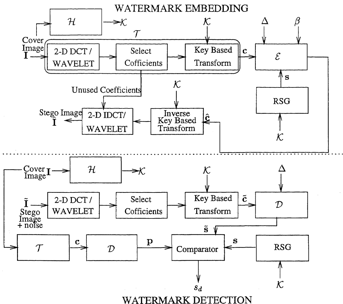
Figure 7.3 Block diagram of the watermark embedding and detection
