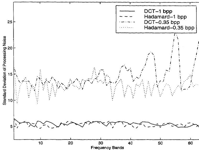
Figure 3.6 Comparison of standard deviations of processing noise for DCT and Hadamard decompositions. The source of processing noise is SPIHT compression at 1 bpp and 0.35 bpp.
