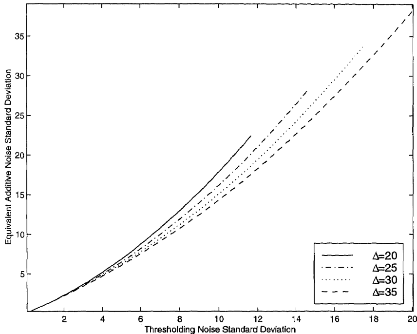
Figure 4.10 Plot of standard deviation of thresholding noise ( \sigma_{st} ) vs standard deviation of equivalent noise due to thresholding, ( \sigma_{st_e} )
