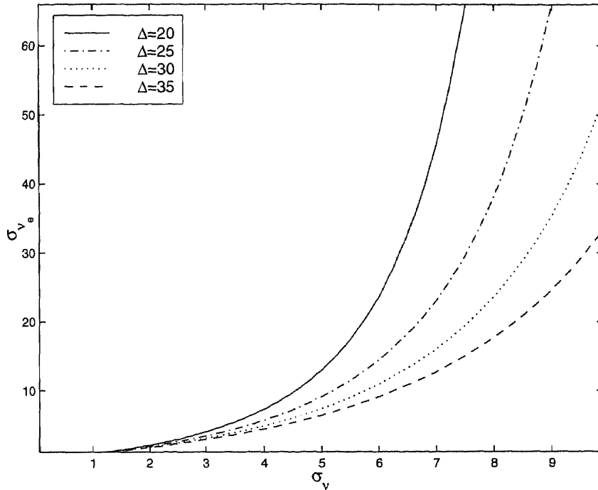
Figure 4.8 Plot of \sigma_{\nu_e}^2 vs \sigma_\nu for \Delta = 20, 25, 30, and 35
