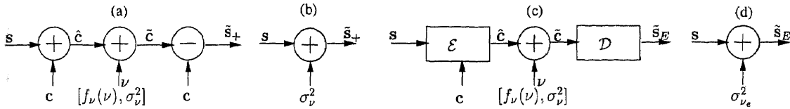
Figure 4.4 (a) Linear non oblivious data hiding. (b) Equivalent additive noise channel. (c) Non-linear oblivious detection data hiding. (d) Equivalent additive noise channel.
