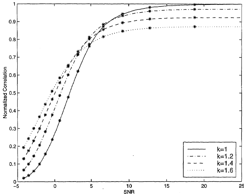
Figure 4.11 Plot of correlation vs SNR for k = 1, 1.2, 1.4 and 1.6
