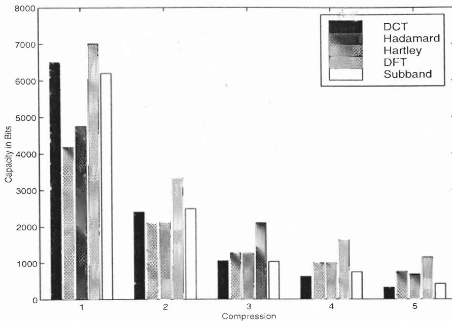
Figure 3.11 Average capacity estimates for 15 images when the message signal has to survive SPIHT or JPEG. The compression indices 1 - 5 correspond to 1 - lossless compression, 2 - (JPEG - 75, SPIHT 1 bpp), 3 - (JPEG - 50, SPIHT 0.75 bpp), 4 - (JPEG - 35, SPIHT 0.5 bpp), 5 - (JPEG - 25, SPIHT 0.35 bpp).
