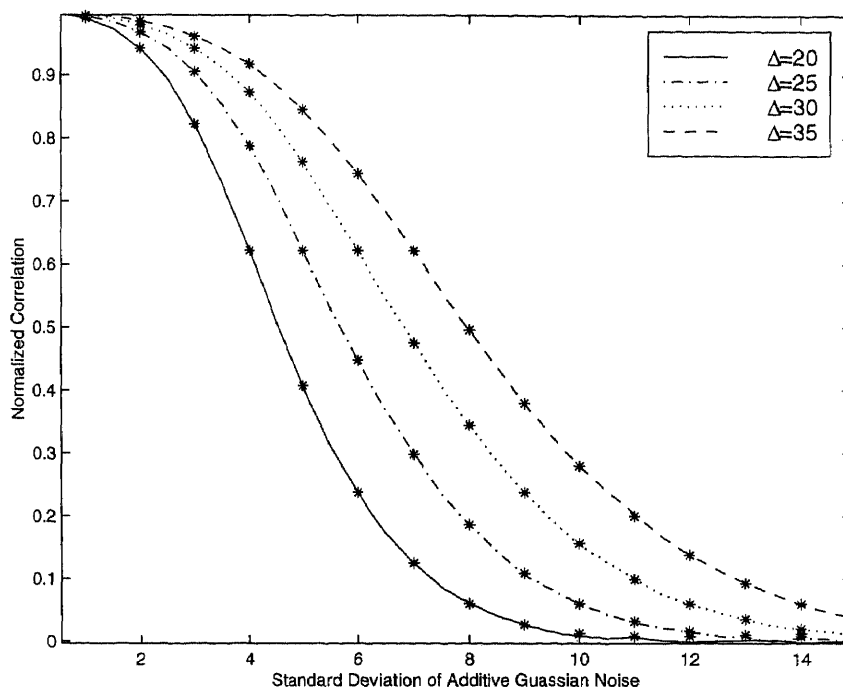
Figure 4.7 Effect of additive Gaussian noise. The lines represent values obtained from simulations. The *s represent the values calculated from Eq. (4.11).
