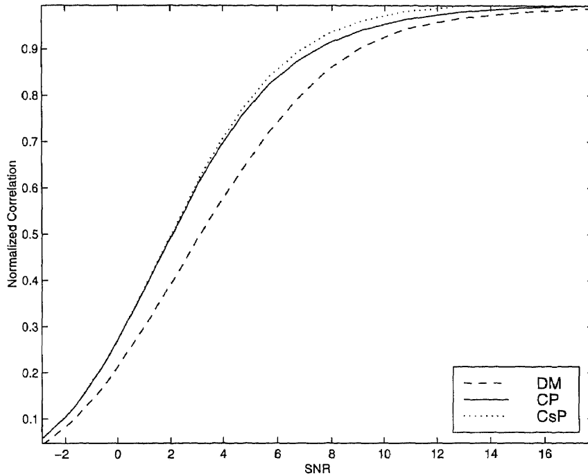
Figure 4.6 Comparison of DM (QIM), CP-SNS and cosine periodic SNS techniques
