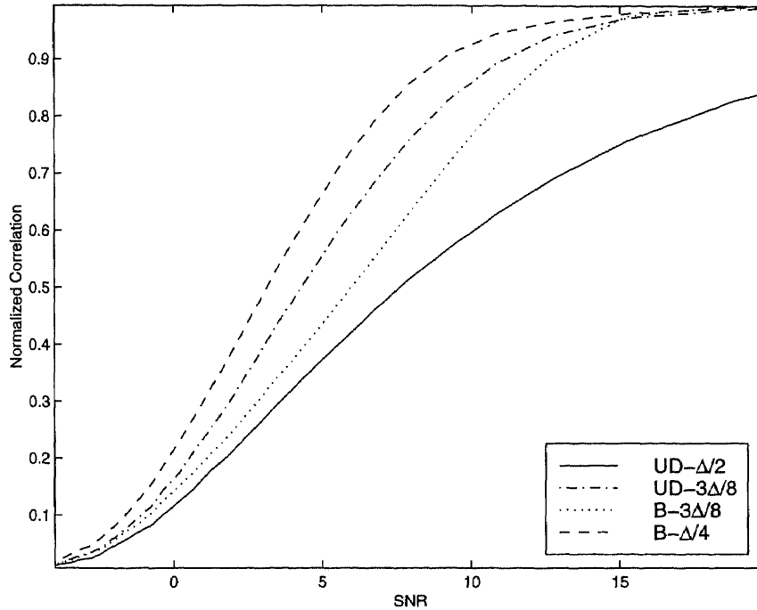
Figure 4.5 Performance of dither modulation for uniformly distributed and binary signature sequences
