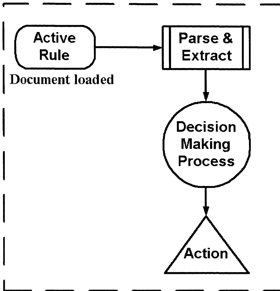
Figure 8 Execution model
