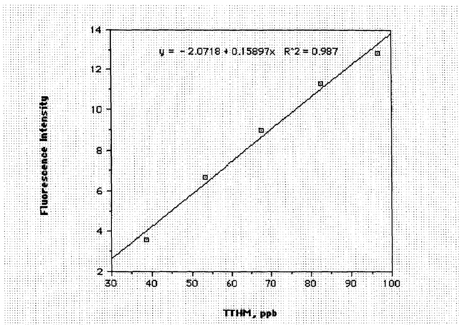
Figure E.1 Fluorescence vs. THMFP, Fluorescence Measured at Excitation Wavelength 250 nm
