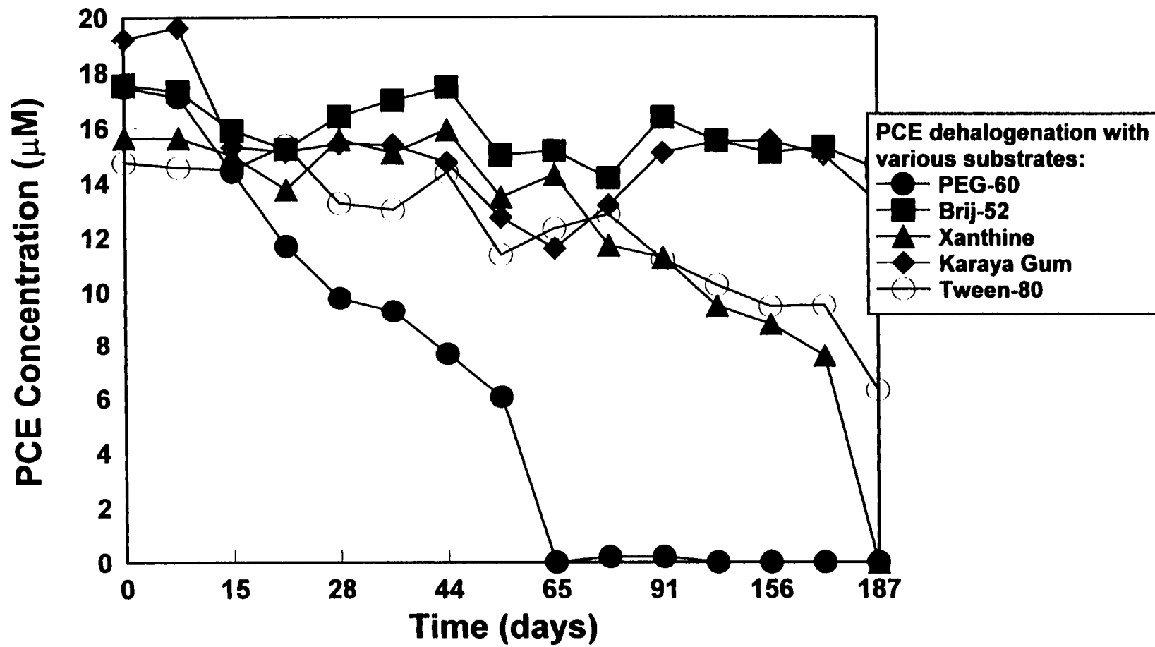
Figure 4.2 Effect of Primary Substrates on the Dehalogenation of Perchloroethylene
