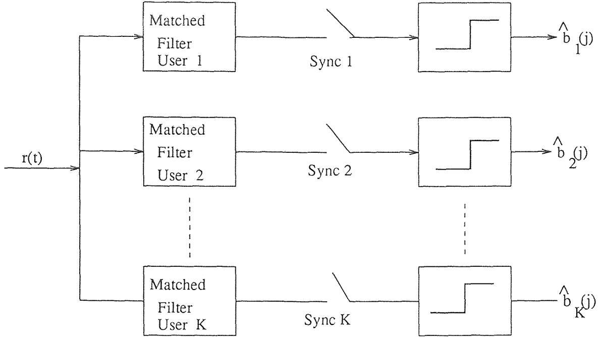
Figure 2.2 Conventional Single User Detector
