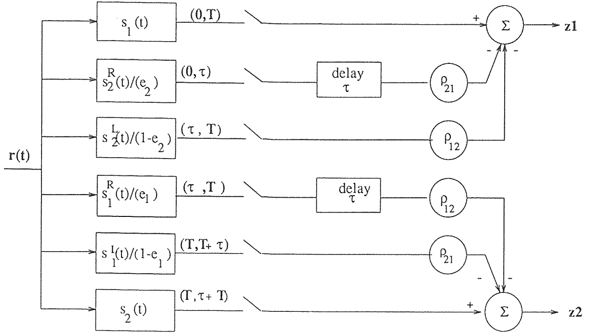
Figure 3.3 Asynchronous Decorrelator
