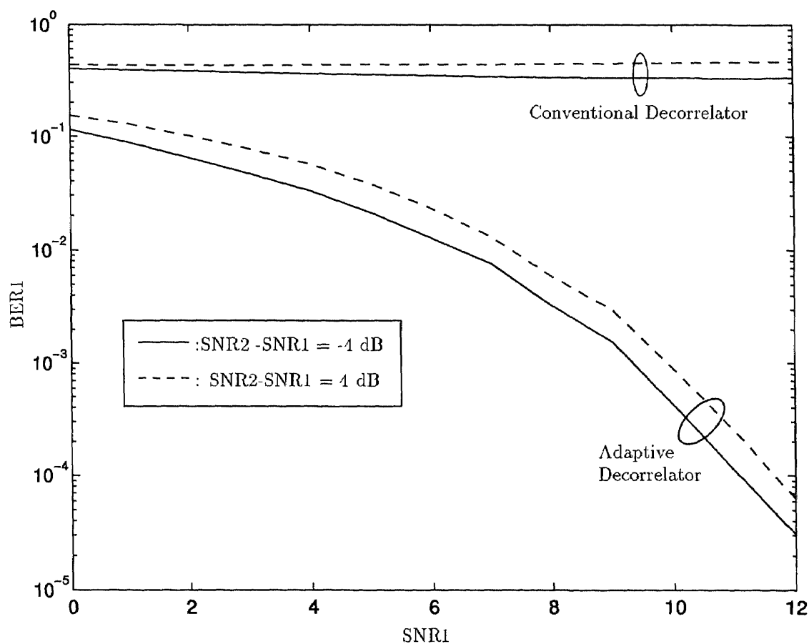
Figure 3.5 Simulated BER performance comparison of the adaptive and non-adaptive decorrelating detectors for fixed interference and variable SNR 1 .
