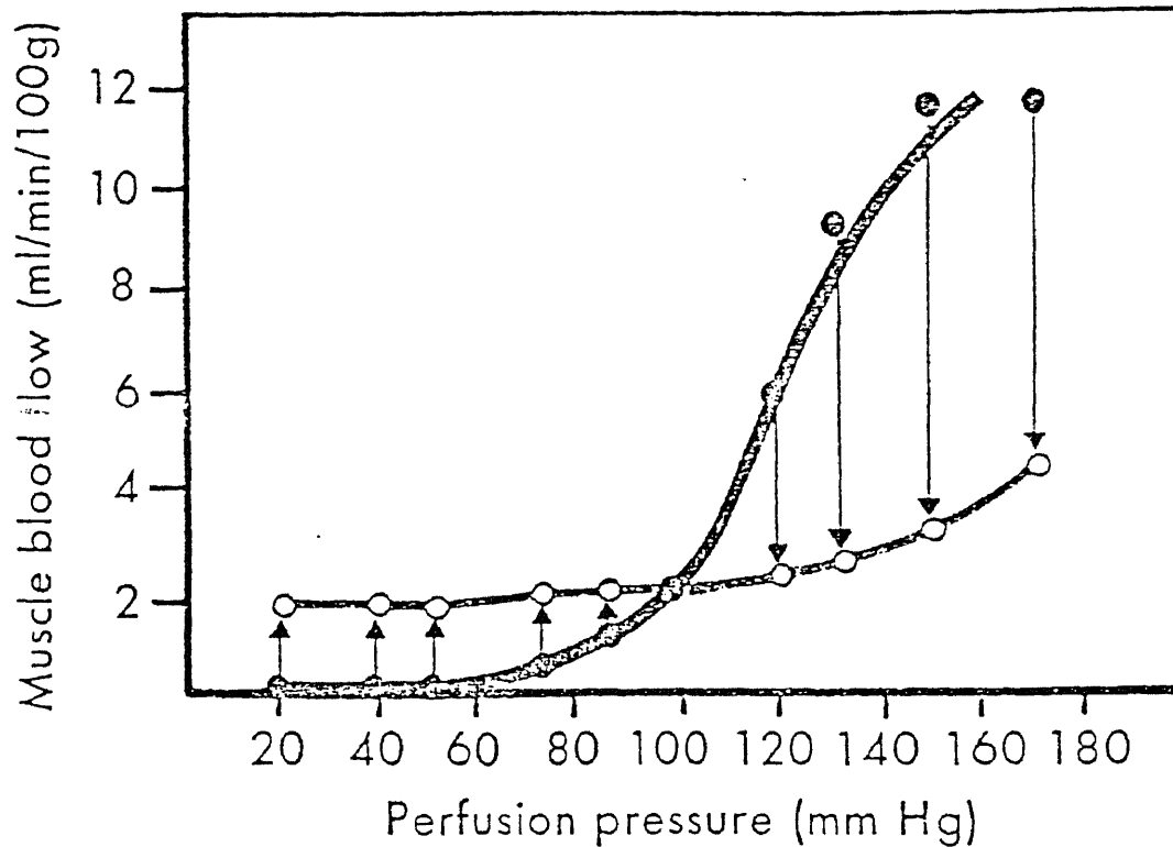
Figure 1.3 Pressure-flow relationship in a certain vascular bed of the dog. The dot represents the flows obtained immediately after abrupt change in perfusion pressure changes from the control level (point where lines cross). The circle represents the steady-state flows obtained at new perfusion pressure.
