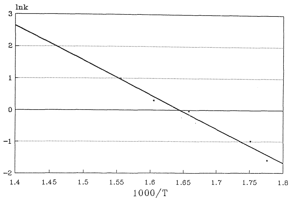
Figure 18 Arrhenius plot of first order rate constant for TCE oxidation 5% \alpha -Fe 2 O 3 / \gamma -Al 2 O 3 / monolith
