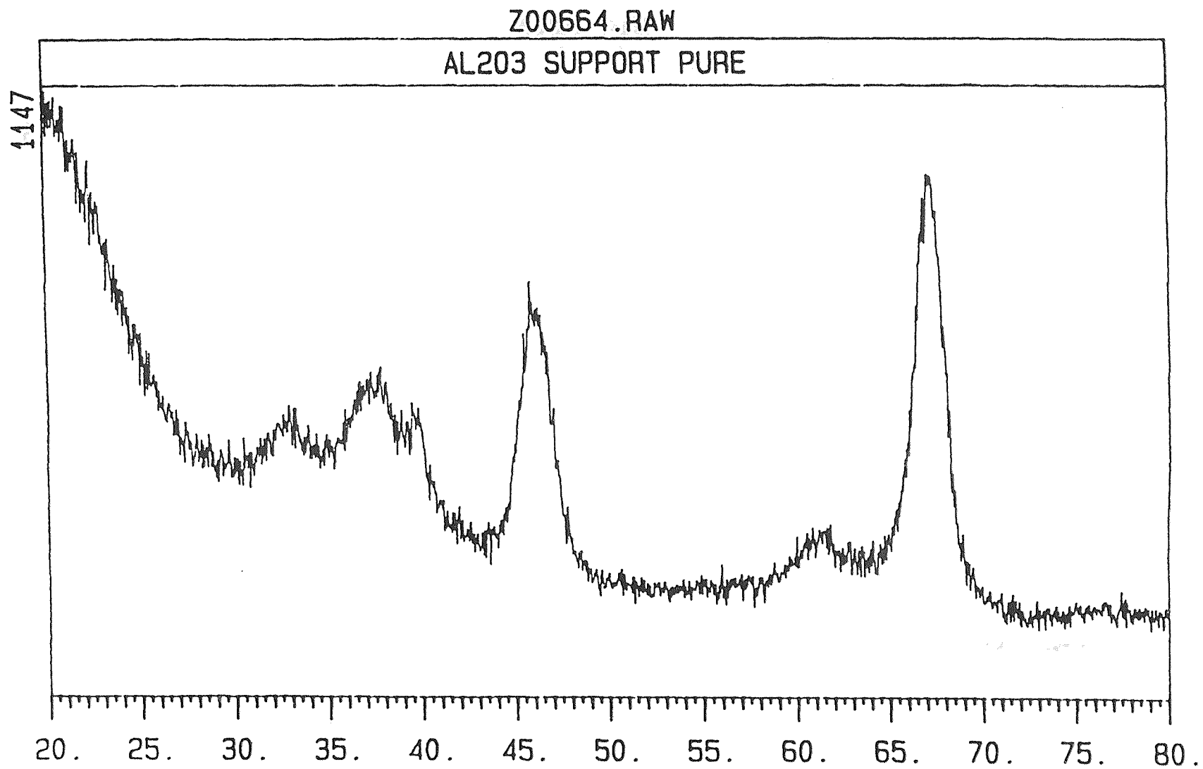
Figure 11 X-Ray Diffraction Spectrum of pure \gamma -Al 2 O 3
