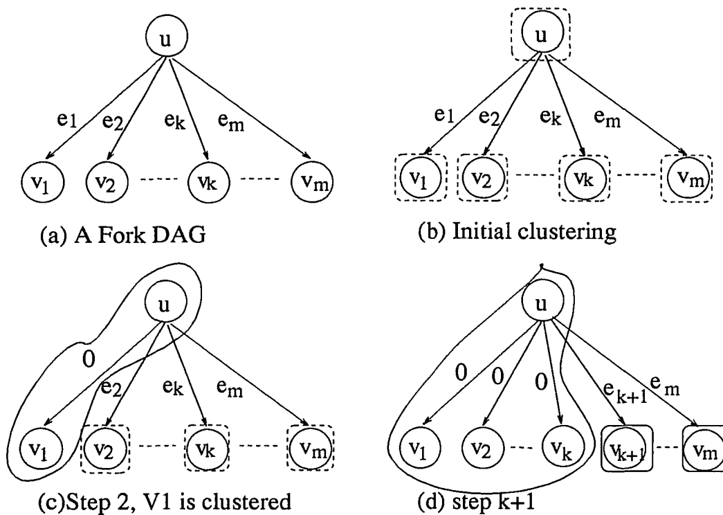
Figure 4.5 CASS-II clustering steps for a fork DAG.
