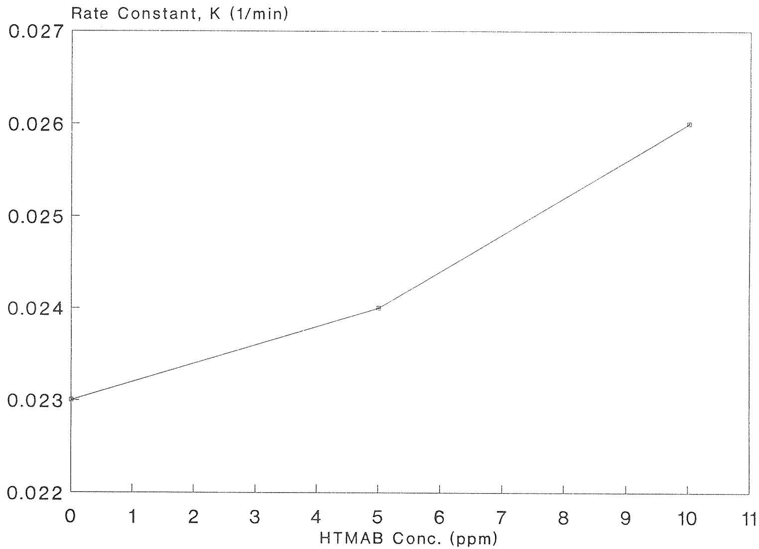
Figure 24 The Effects of HTMAB Concentration on Rate Constant.
