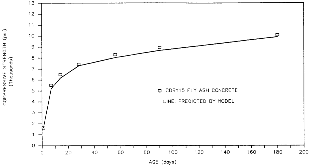
Figure 5.73 Compressive Strength of the Original Feed of Dry Bottom Fly Ash Concrete Predicted by the Proposed Model (15% Replacement)
