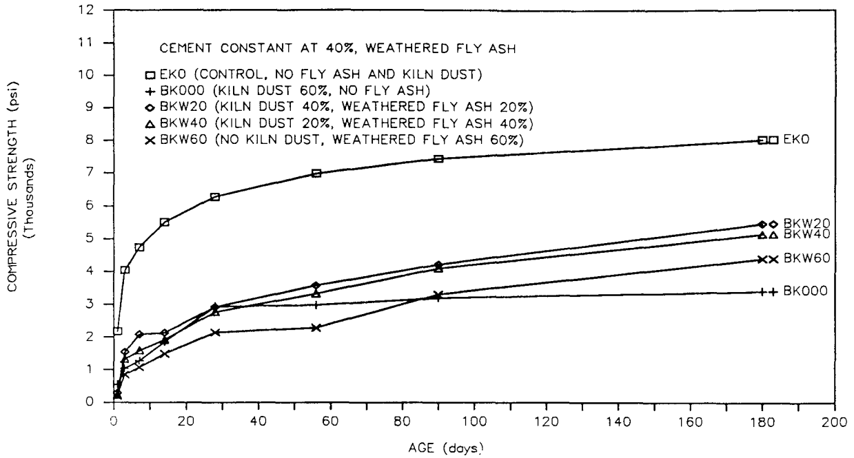
Figure 5.22 Effect of the Weathered Fly Ash-Kiln Dust on the Strength of Mortar with Cement Constant at 40%
