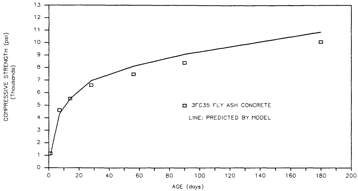
Figure A 3 Compressive Strength of the Fractionated 3F Fly Ash Concrete Predicted by the Proposed Model (35% Replacement)
