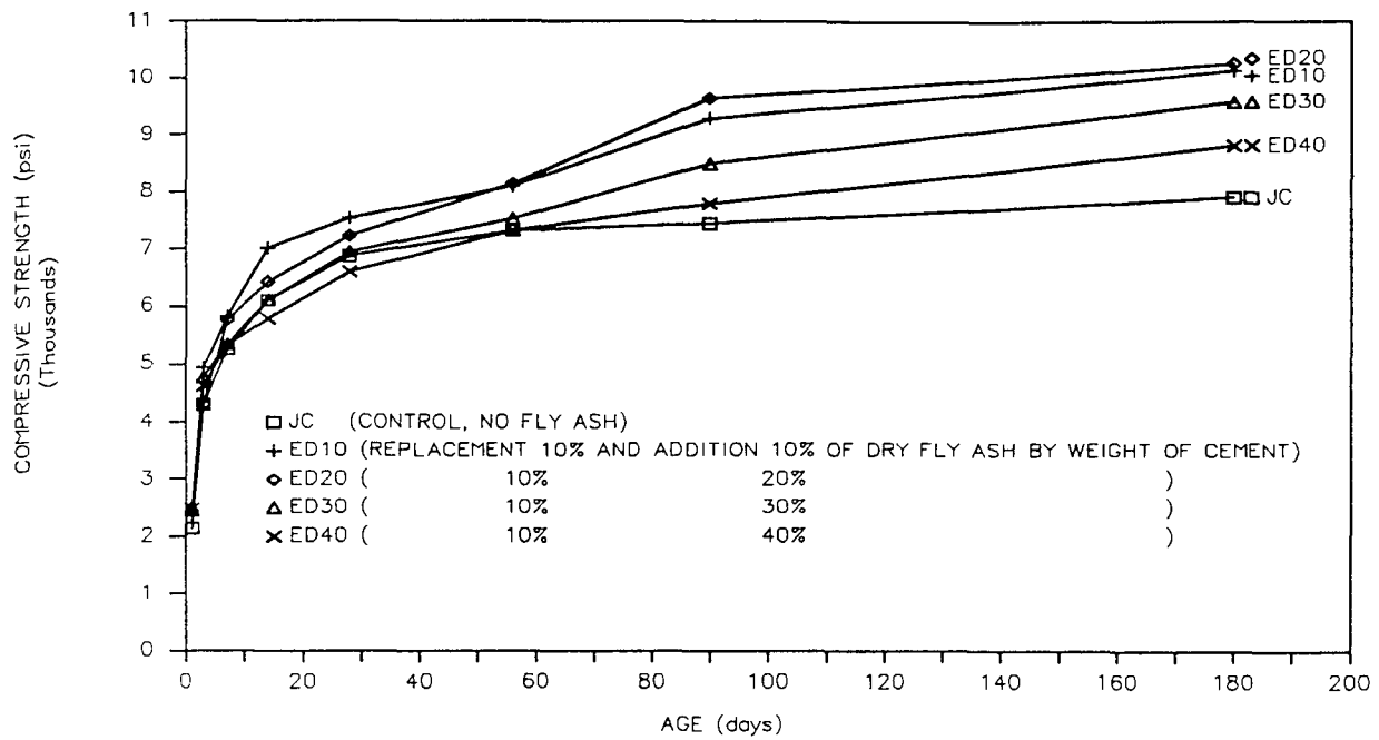
Figure 5.31 Effect of the Dry Fly Ash as a Partial Addition and Replacement of Sand on the Strength of Mortar
