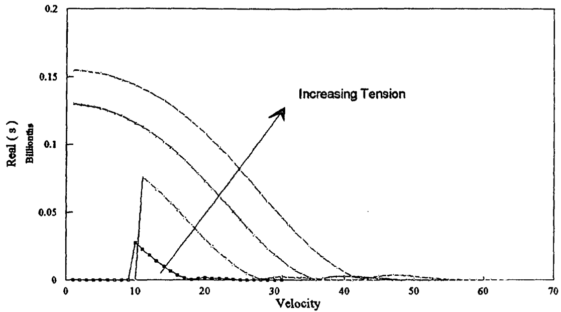
Figure 17 Real part of the First Eigenvalue versus Velocity, Simple-Simple Support
