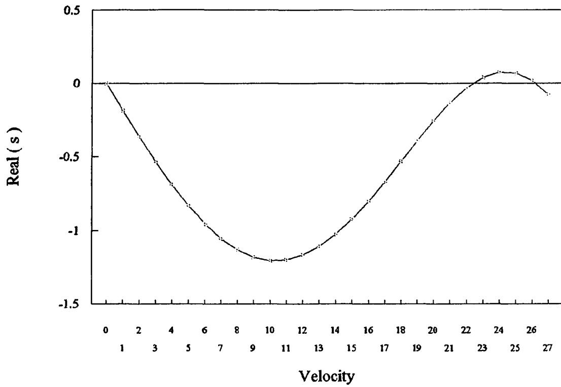
Figure 23 Real part of the Eigenvalue versus Velocity at Tension=750 Fixed-Simple Support
