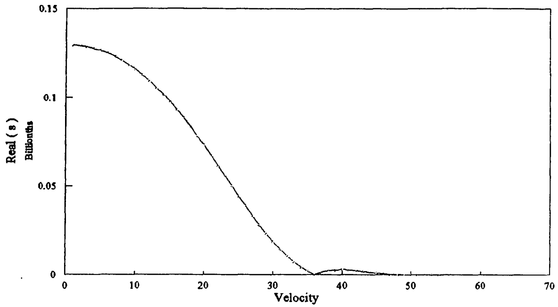
Figure 13 Real part of the First Eigenvalue versus Velocity at Tension=3000 Simple-Simple Support
