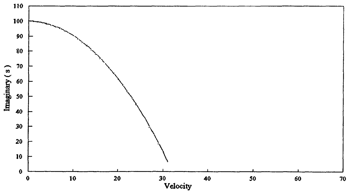
Figure 10 Imaginary part of the Eigenvalue versus Velocity at Tension=1000 Simple-Simple Support
