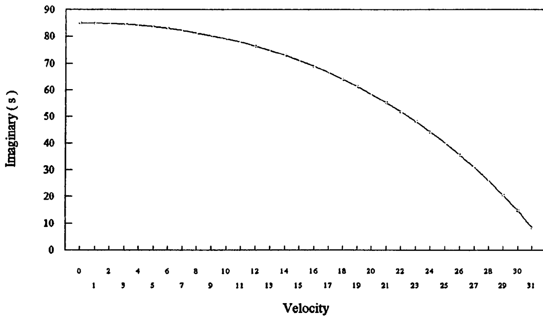
Figure 26 Imaginary part of the Eigenvalue versus Velocity at Tension=1000 Fixed-Simple Support
