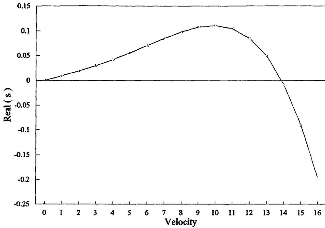
Figure 19 Real part of the Eigenvalue versus Velocity at Tension=250 Fixed-Simple Support
