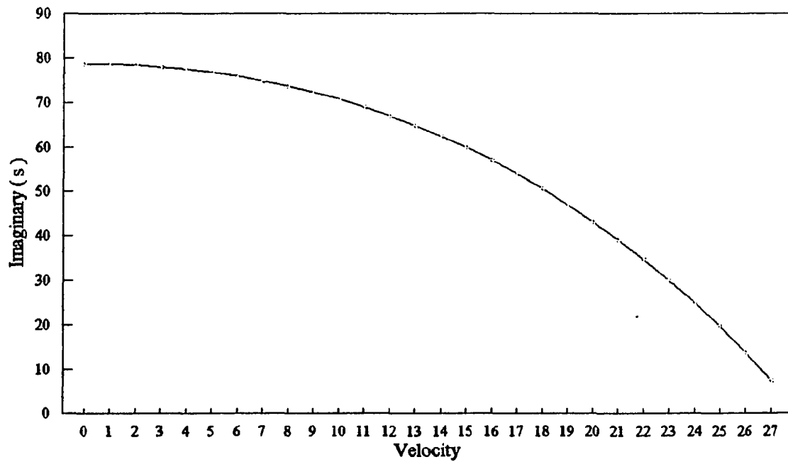
Figure 24 Imaginary part of the Eigenvalue versus Velocity at Tension=750 Fixed-Simple Support
