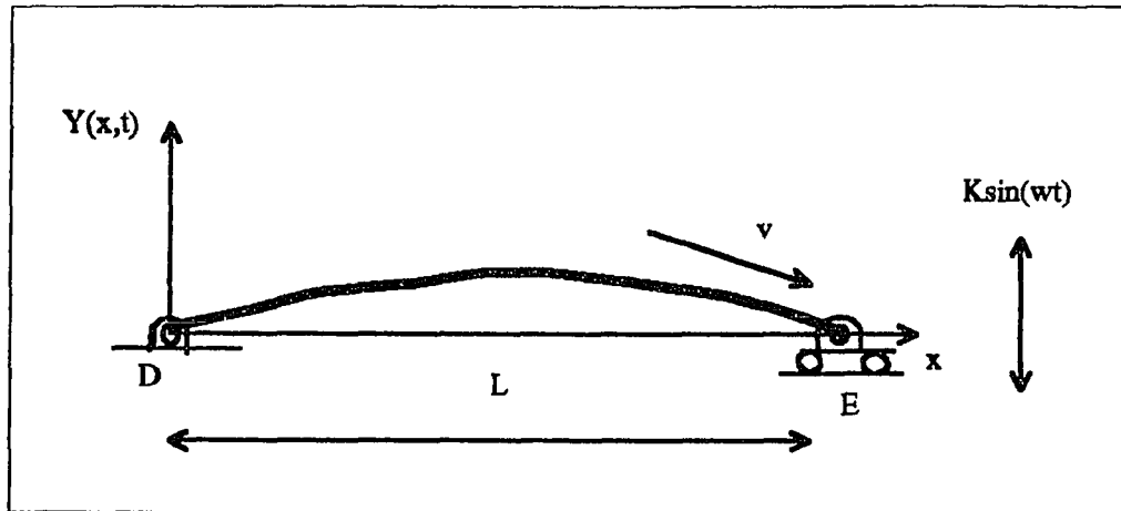
Figure 4 The Axially Moving Bernoulli-Euler Beam Under Tension
