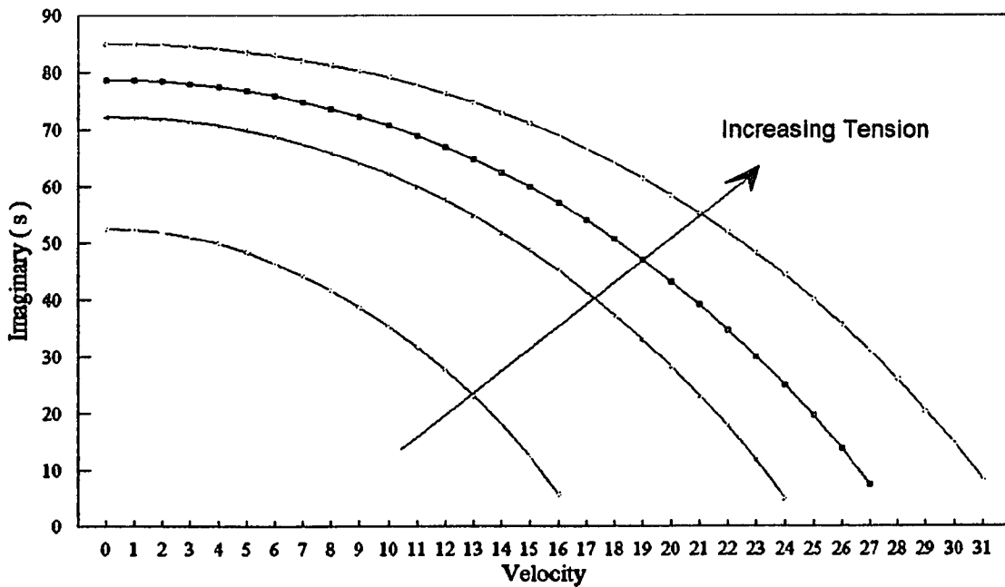
Figure 28 Imaginary part of the Eigenvalue versus Velocity , Fixed-Simple Support
