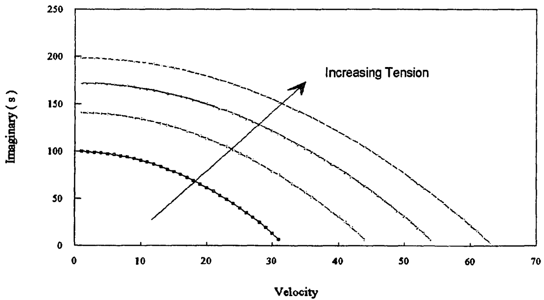
Figure 18 Imaginary part of the Eigenvalue versus Velocity, Simple-Simple Support
