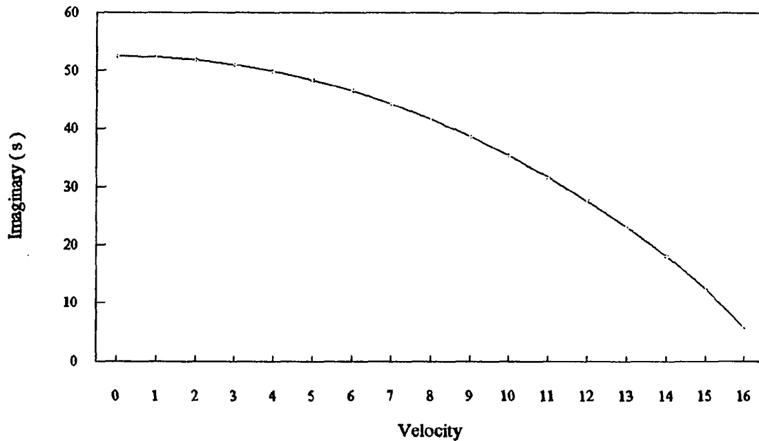
Figure 20 Imaginary part of the Eigenvalue versus Velocity at Tension=250 Fixed-Simple Support
