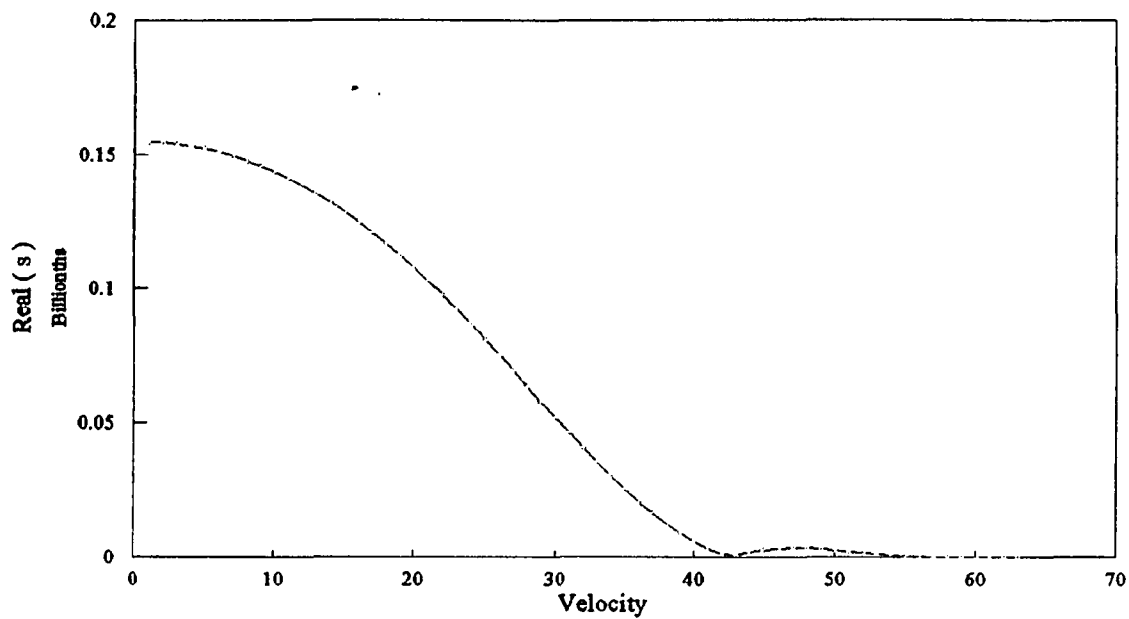
Figure 15 Real part of the First Eigenvalue versus Velocity at Tension=4000 Simple-Simple Support
