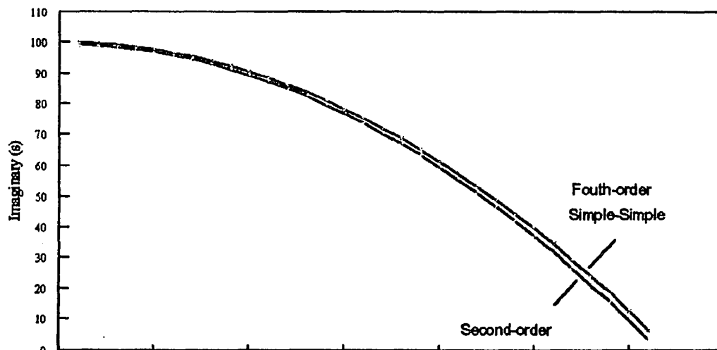
Figure 8 The Comparison between Second-order Model and the Fourth-order Model with Simple-Simple Supports
