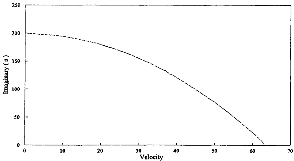
Figure 16 Imaginary part of the Eigenvalue versus Velocity at Tension=4000 Simple-Simple Support
