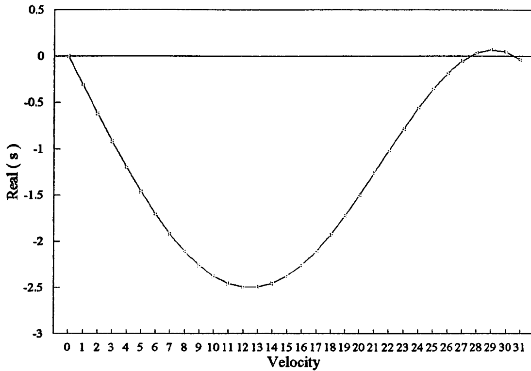
Figure 25 Real part of the Eigenvalue versus Velocity at Tension=1000 Fixed-Simple Support
