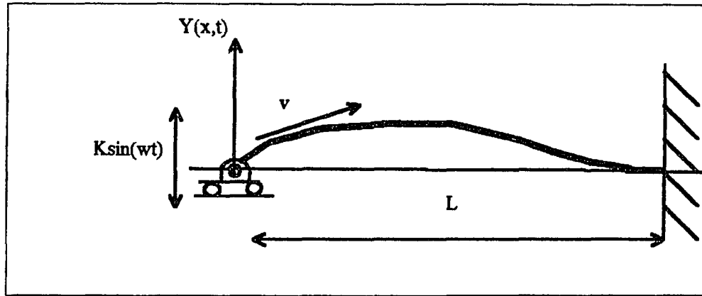
Figure 5 The Fixed-Simple Support Beam Model For segments AC and BC in Figure 1
