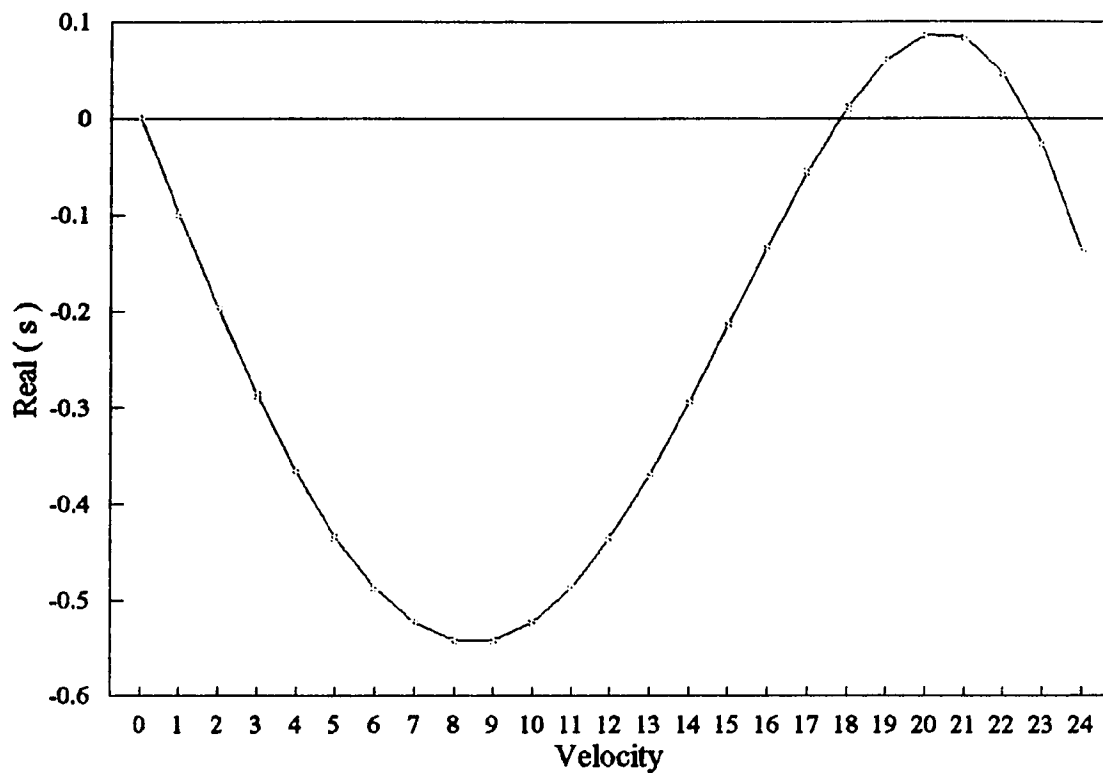
Figure 21 Real part of the Eigenvalue versus Velocity at Tension=575 Fixed-Simple Support
