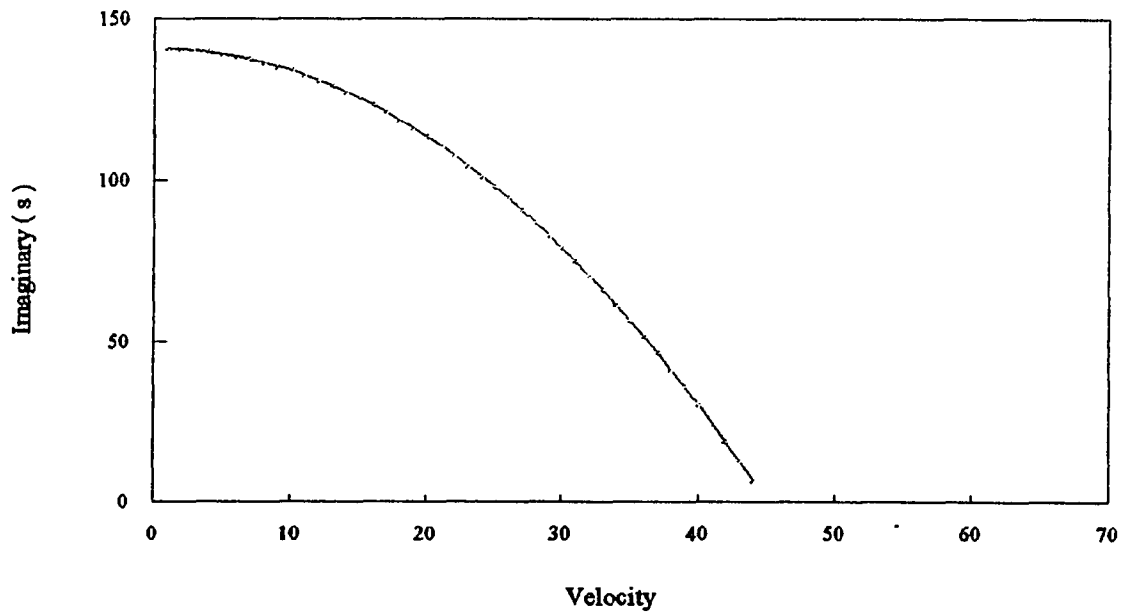
Figure 12 Imaginary part of the Eigenvalue versus Velocity at Tension=2000 Simple-Simple Support
