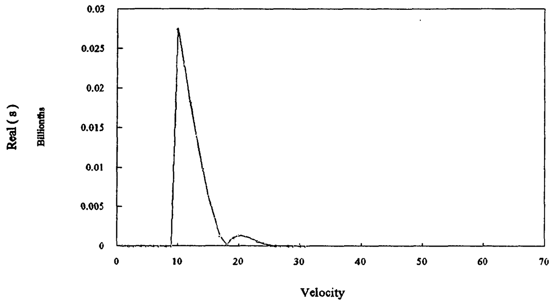
Figure 9 Real part of the First Eigenvalue versus Velocity at Tension=1000 Simple-Simple Support
