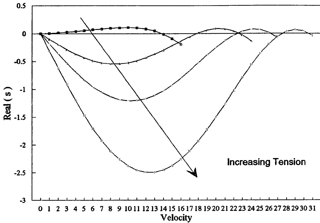
Figure 27 Real part of the Eigenvalue versus Velocity , Fixed-Simple Support
