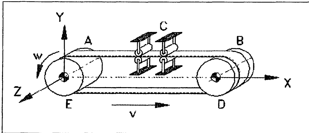
Figure 1 Schematic Band-Saw Assembly
