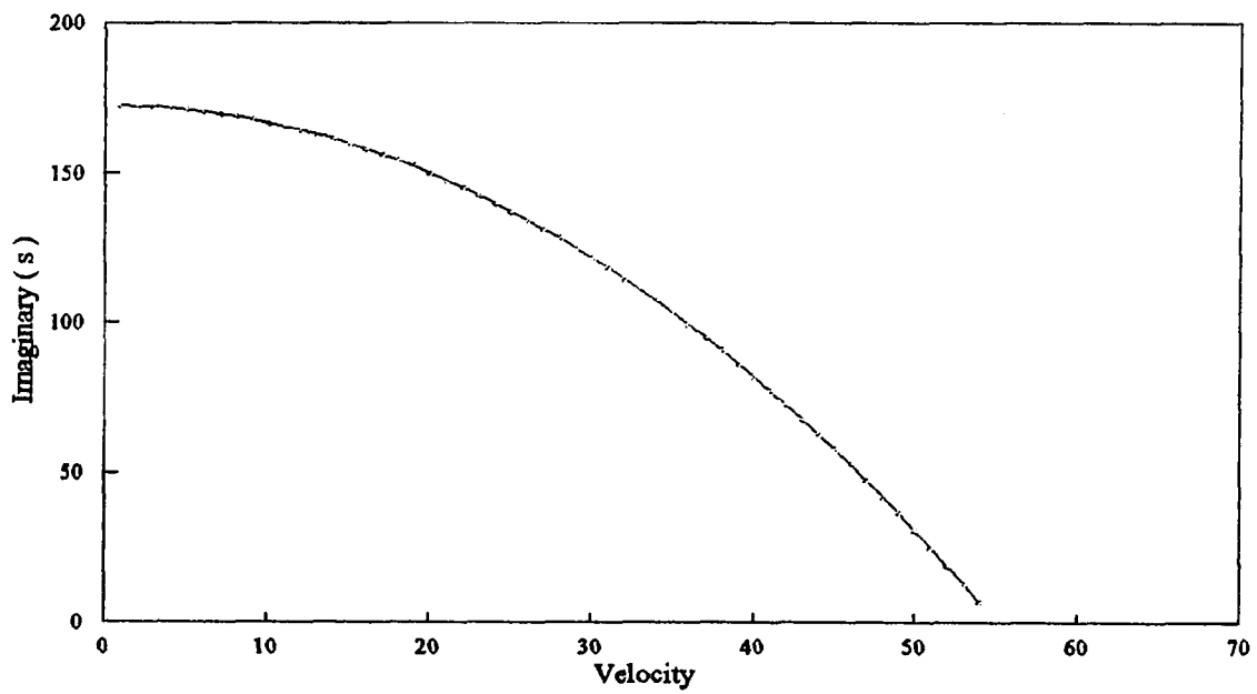
Figure 14 Imaginary part of the Eigenvalue versus Velocity at Tension=3000 Simple-Simple Support
