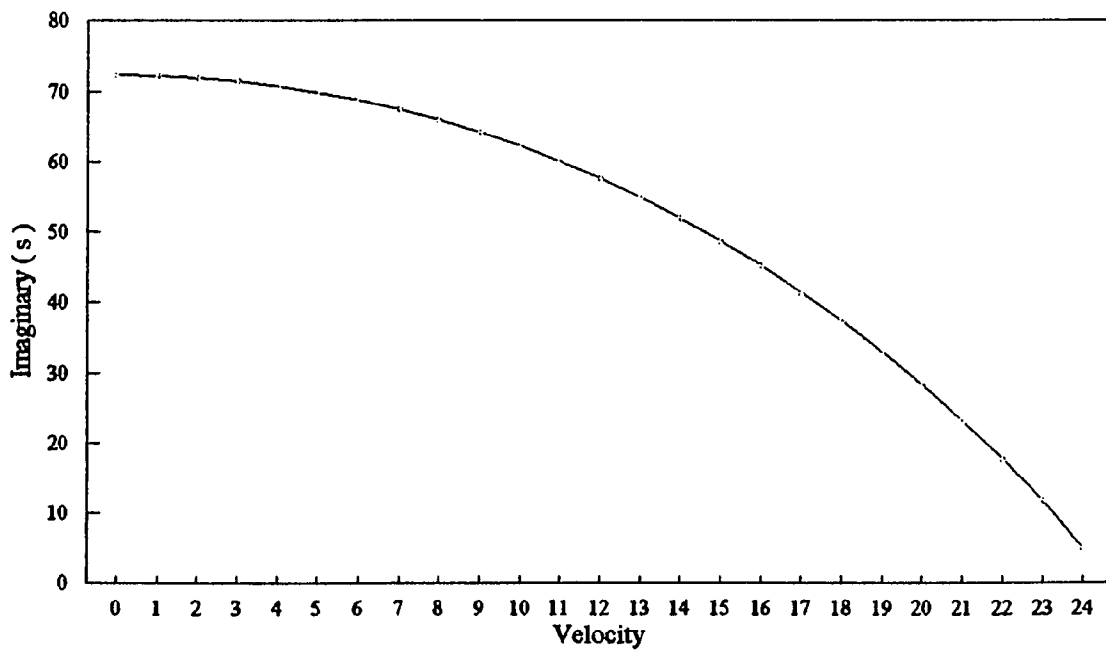
Figure 22 Imaginary part of the Eigenvalue versus Velocity at Tension=575 Fixed-Simple Support
