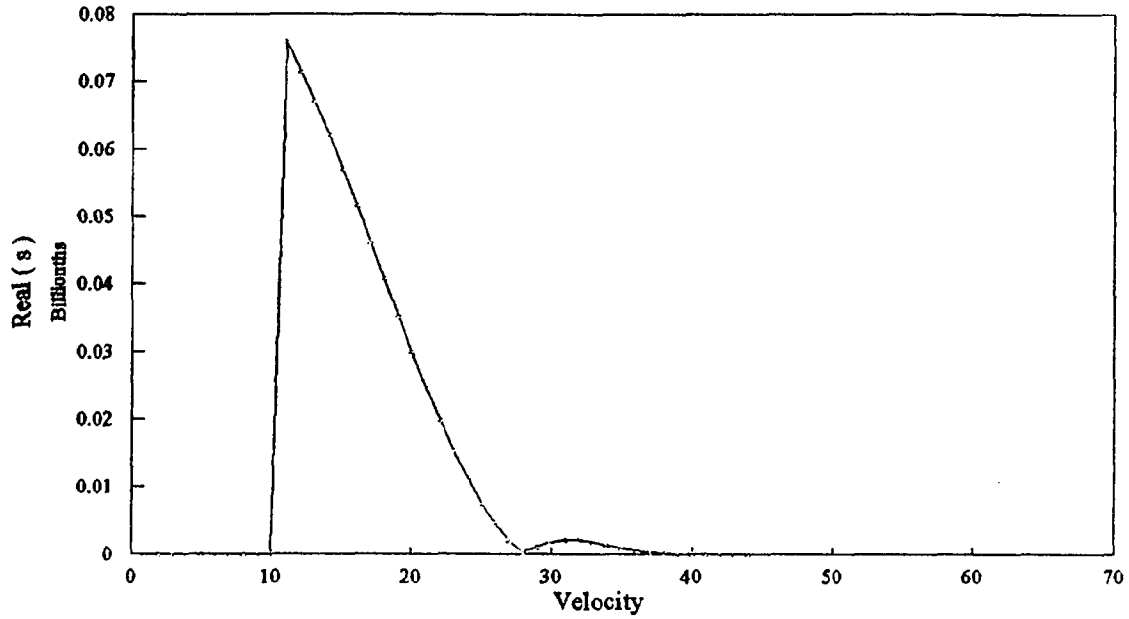
Figure 11 Real part of the First Eigenvalue versus Velocity at Tension=2000 Simple-Simple Support
