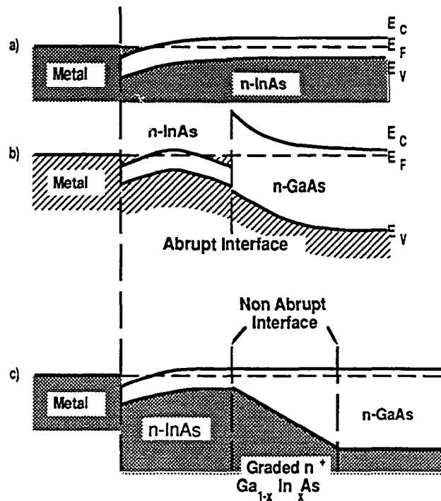
Figure 2.19: Band diagram of a non-alloyed ohmic contact to n-GaAs (a) Shows that any metal can make ohmic contact to n-InAs (b) Abrupt interface of n-InAs/n-GaAs due to conduction band discontinuity (c) A graded n-In x Ga 1-x As layer makes ohmic contact to n-GaAs
