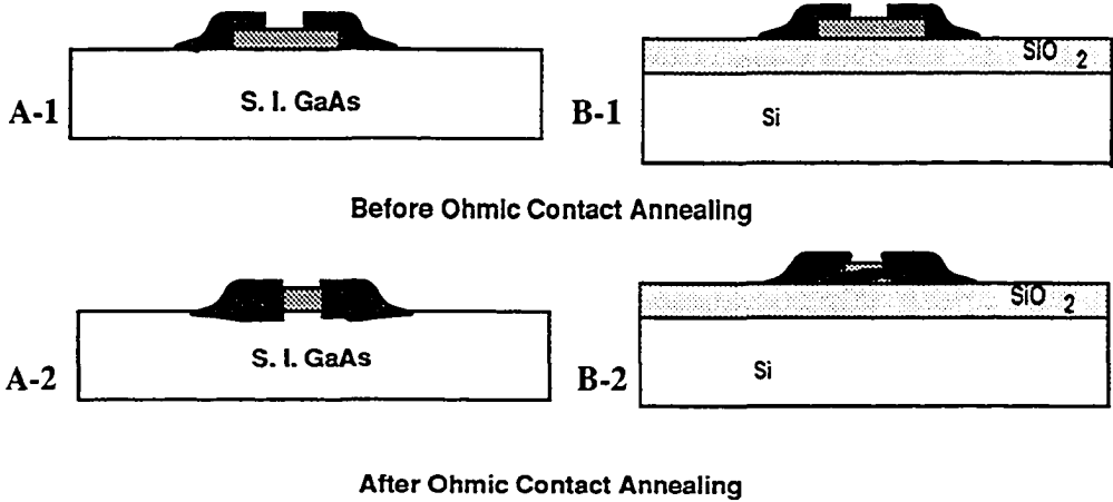
Figure 2.17: Illustration of AuGe ohmic contact alloy flow
