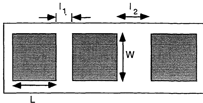
Figure 2.1(a): A transmission line pattern for ohmic contact resistance evaluation
