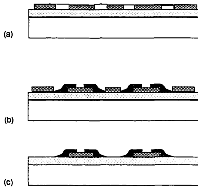
Figure 2.16: Cross sectional view of the altered FET process shown in Figure 2.15 (a) Hole etch next to 'future mesa' site (b) Ohmic metal deposition (c) Mesa isolation
