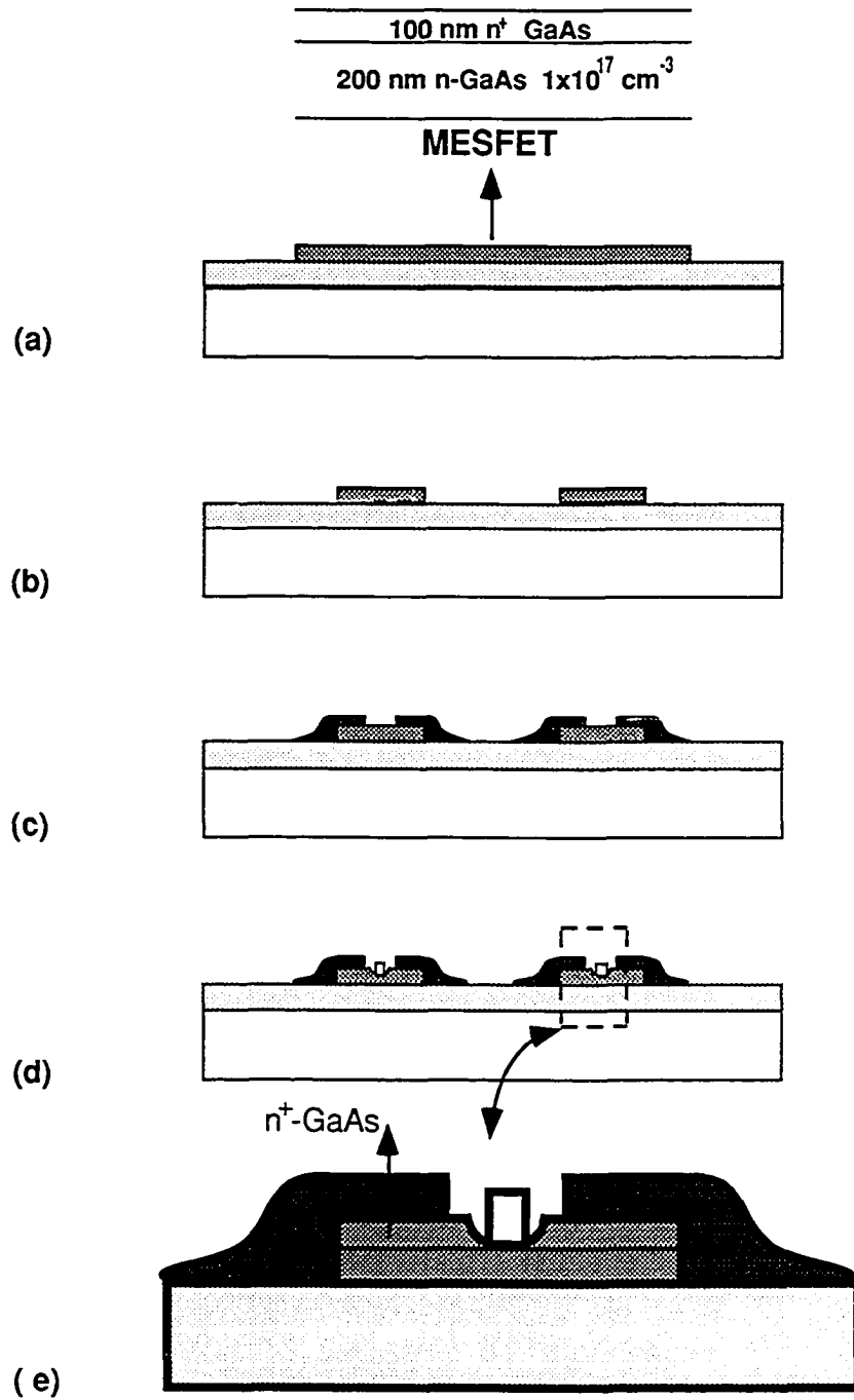
Figure 2.4: ELO GaAs FET process sequence
