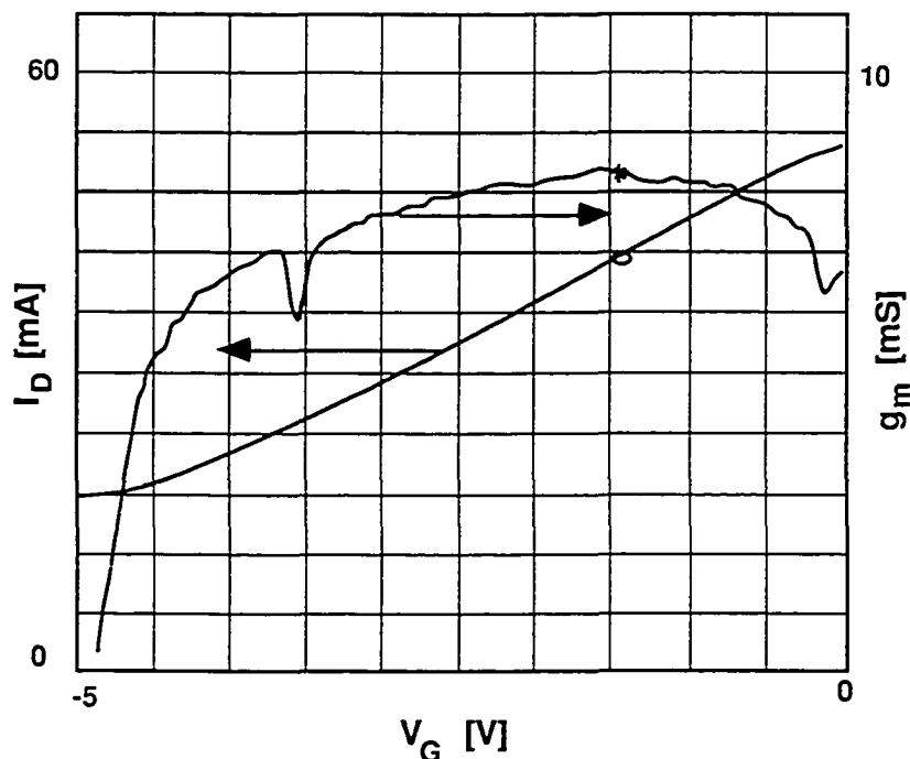
Figure 2.23(a): DC transfer characteristics of an ELO GaAs MESFET on \text{SiO}_2/\text{Si} with alloyed contacts and without recessed gate. I_{\text{dss}} = 260 \text{ mA/mm} , g_{\text{m-max}} = 41.5 \text{ mS/mm} . Gate width W_{\text{g}} = 200 \text{ } \mu\text{m} .
