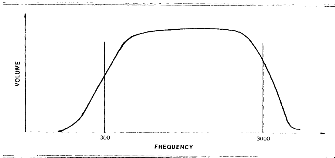
Figure 3.1. The Bandwidth of a Public Telephone Line
