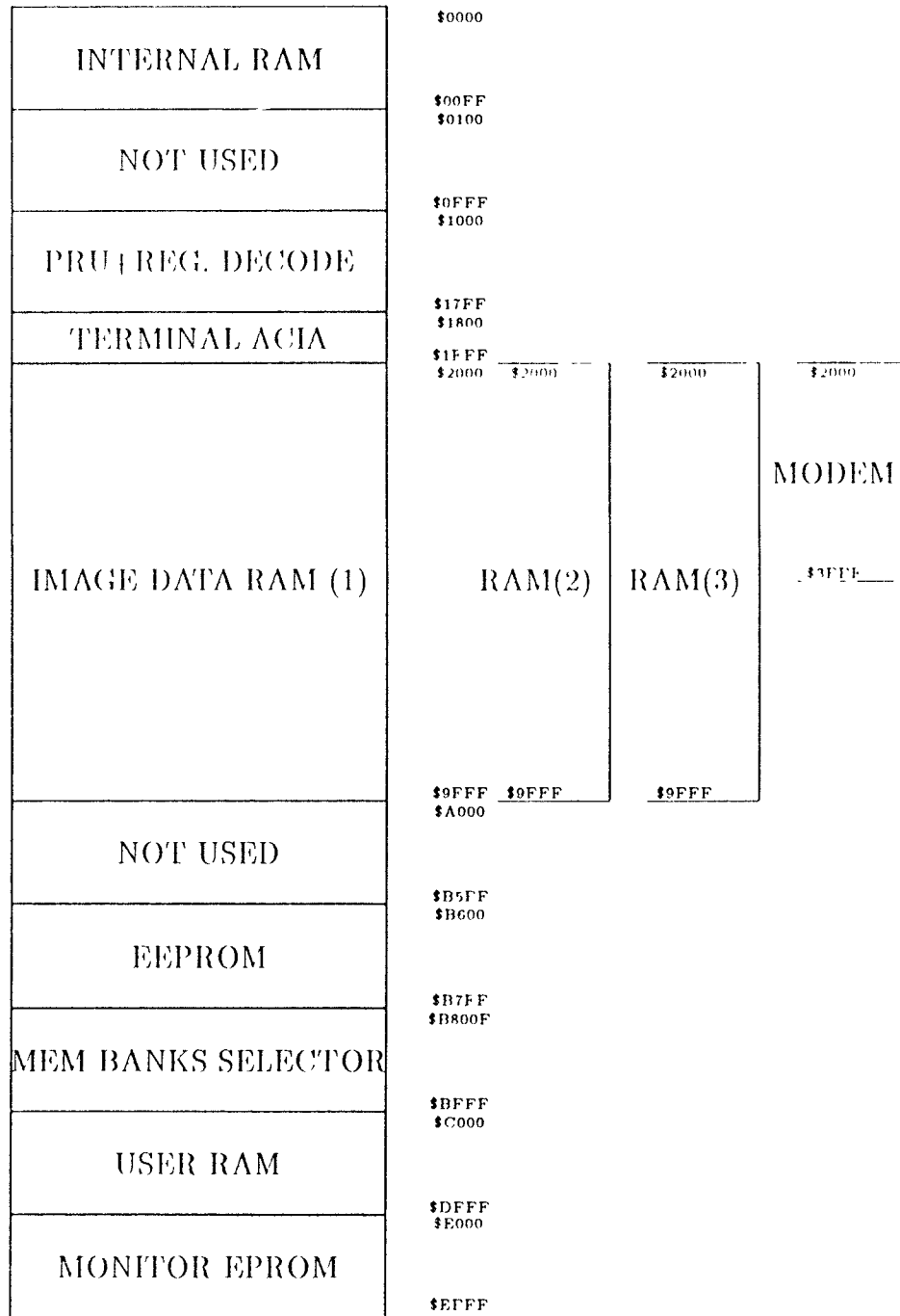
Figure 4.2: EVB New Memory Map Diagram
