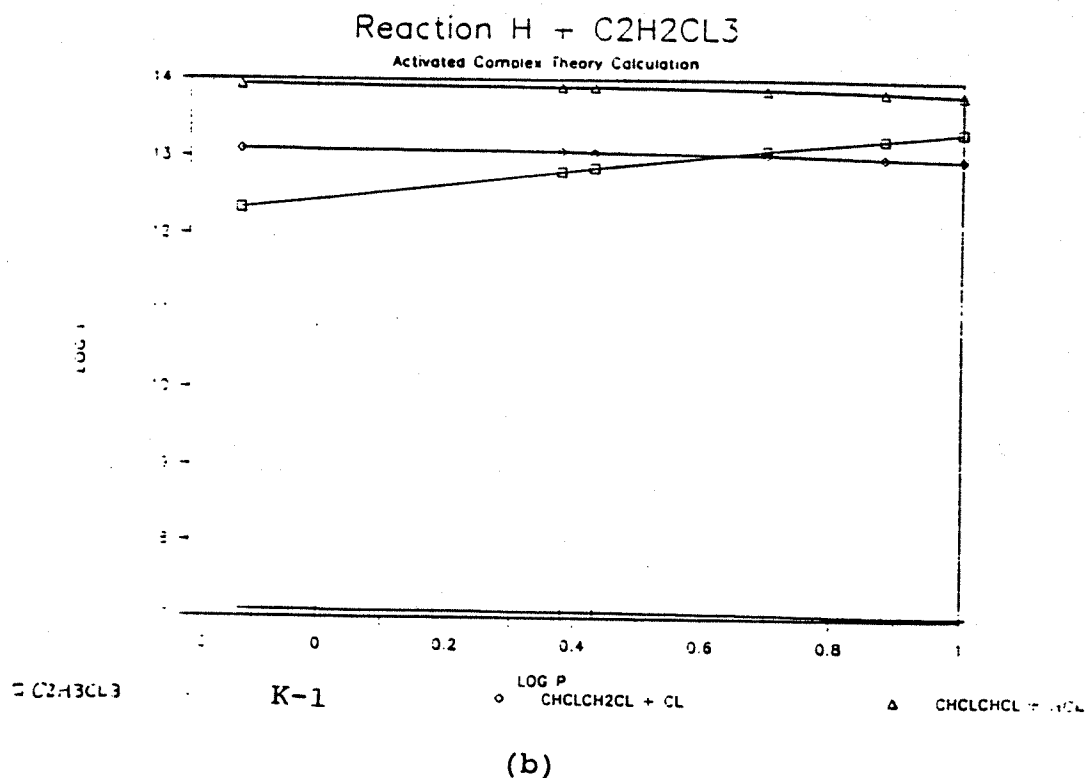
Figure 9 . Energy Diagram (a) and CHEMACT Results (b) for Reaction H + C 2 H 2 Cl 3
