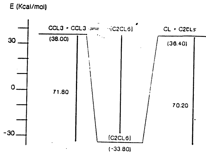
ENERGY DIAGRAM : CCL_3 + CCL_3
