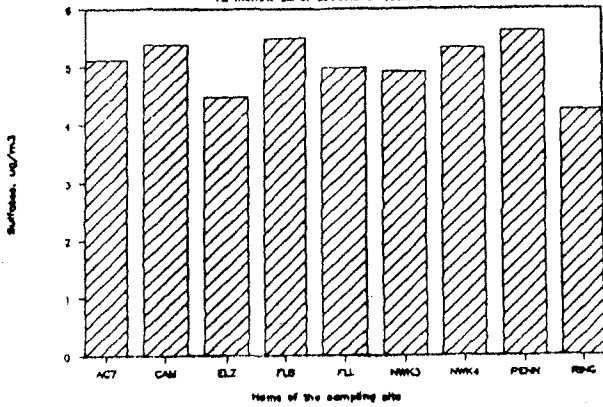
Sulfates, ug/m3
