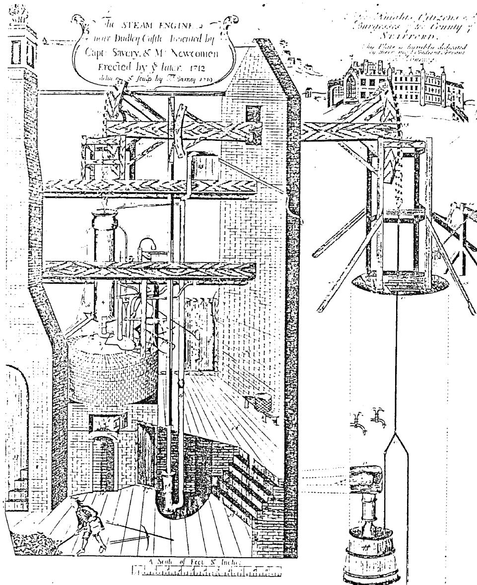
52 The Newcomen engine at Dudley Castle engraved by Thomas Barneij, 1719. Crown Copyright, Science Museum, London
