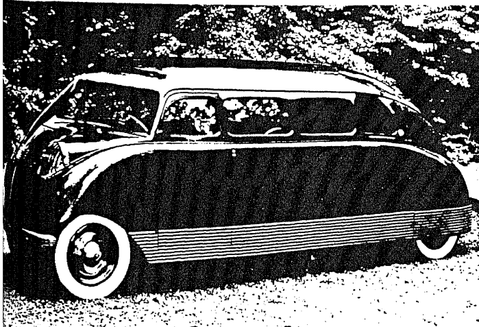
The earlier Stout Scarab had a steel body on a steel hoop chassis and boasted exceptional interior space
