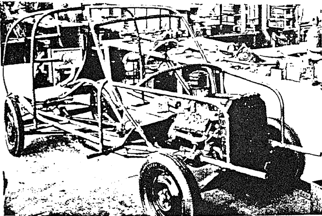
Had's soybean car had tubular frame and fourteen surface steel. He bought acreage in Dearborn to grow the beans for it.
