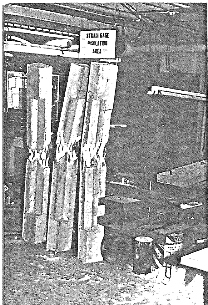
Figure 3.38 - CRACK PATTERNS
