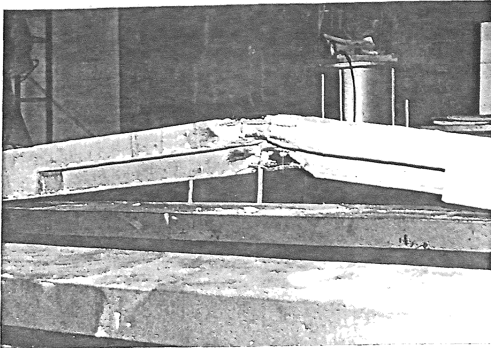
Figure 3.43 - CRACK PATTERNS
