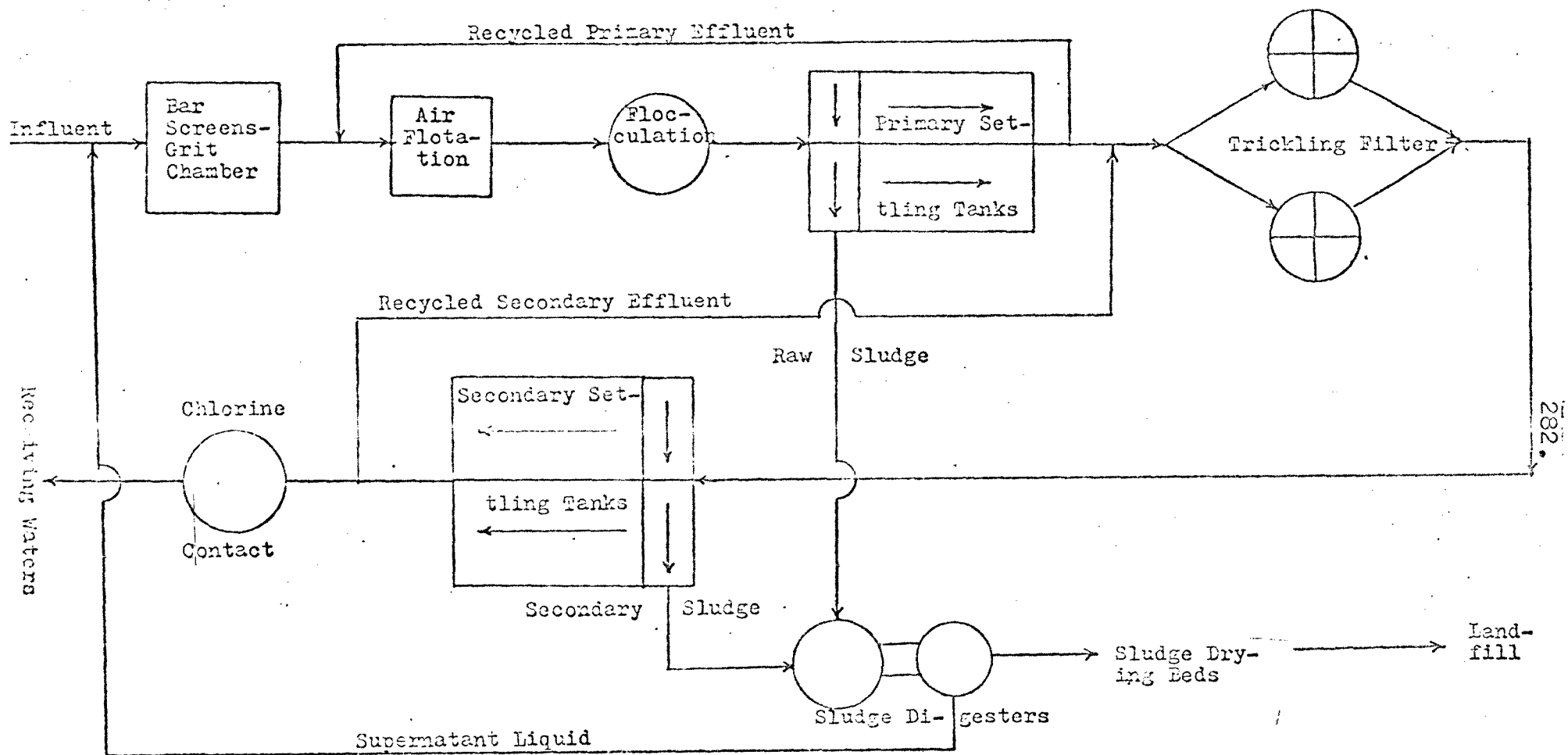
FIGURE NO. 32 UP-GRADED KEARNY TREATMENT PLANT
