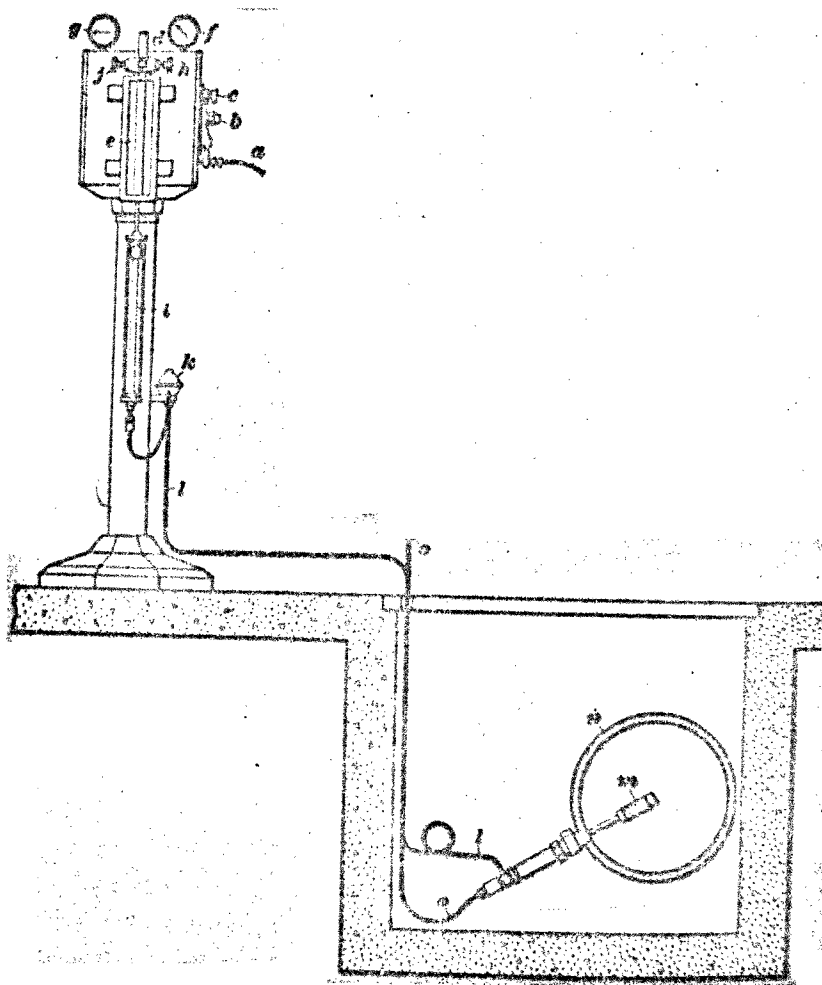
Fig. 20. Wallace and Tiernan Direct-Feed Chlorinator.
