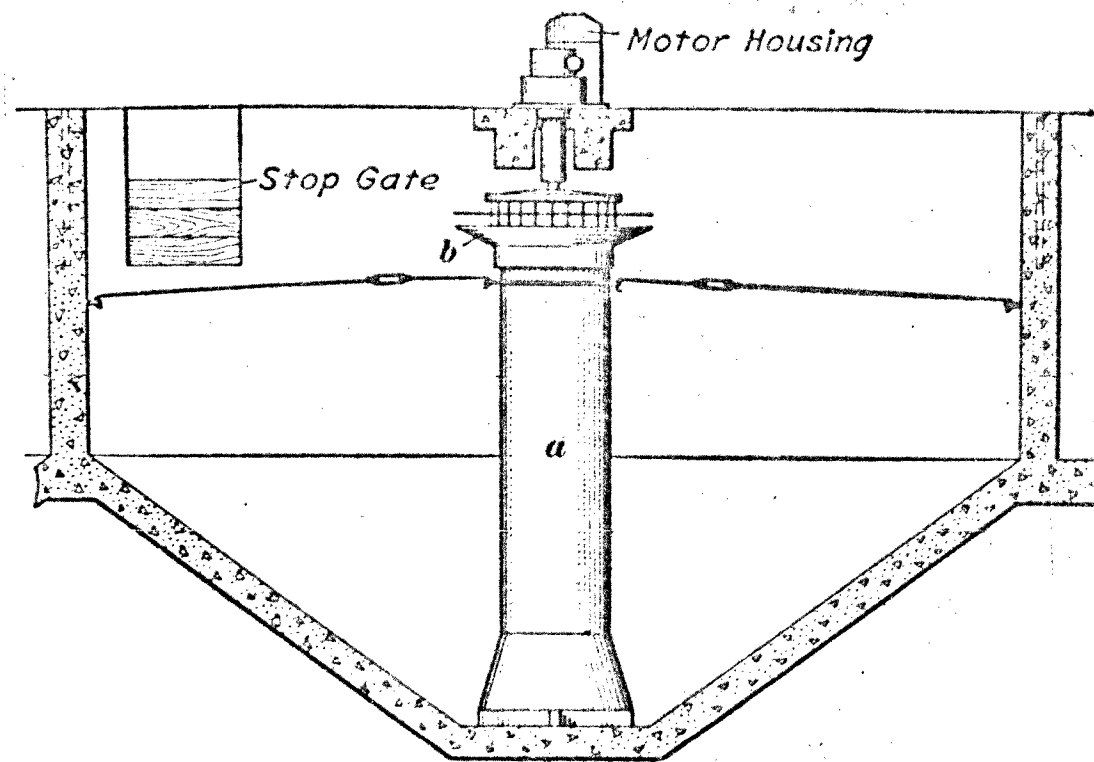
Fig. 12. Simplex Mechanical Aerator.
