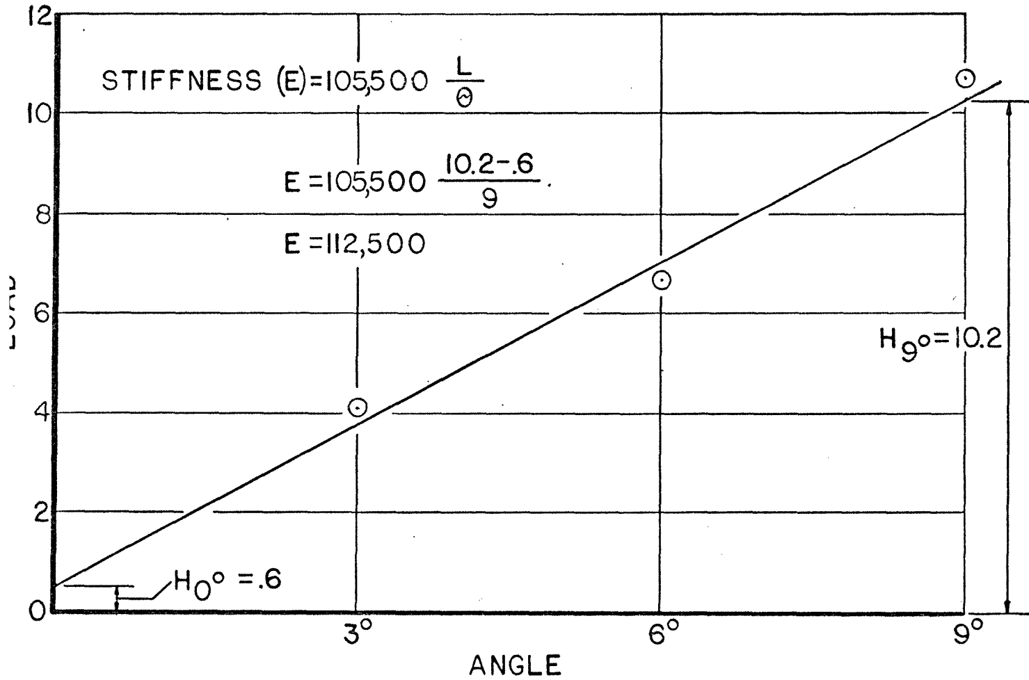
FIGURE 6 STIFFNESS TEST
