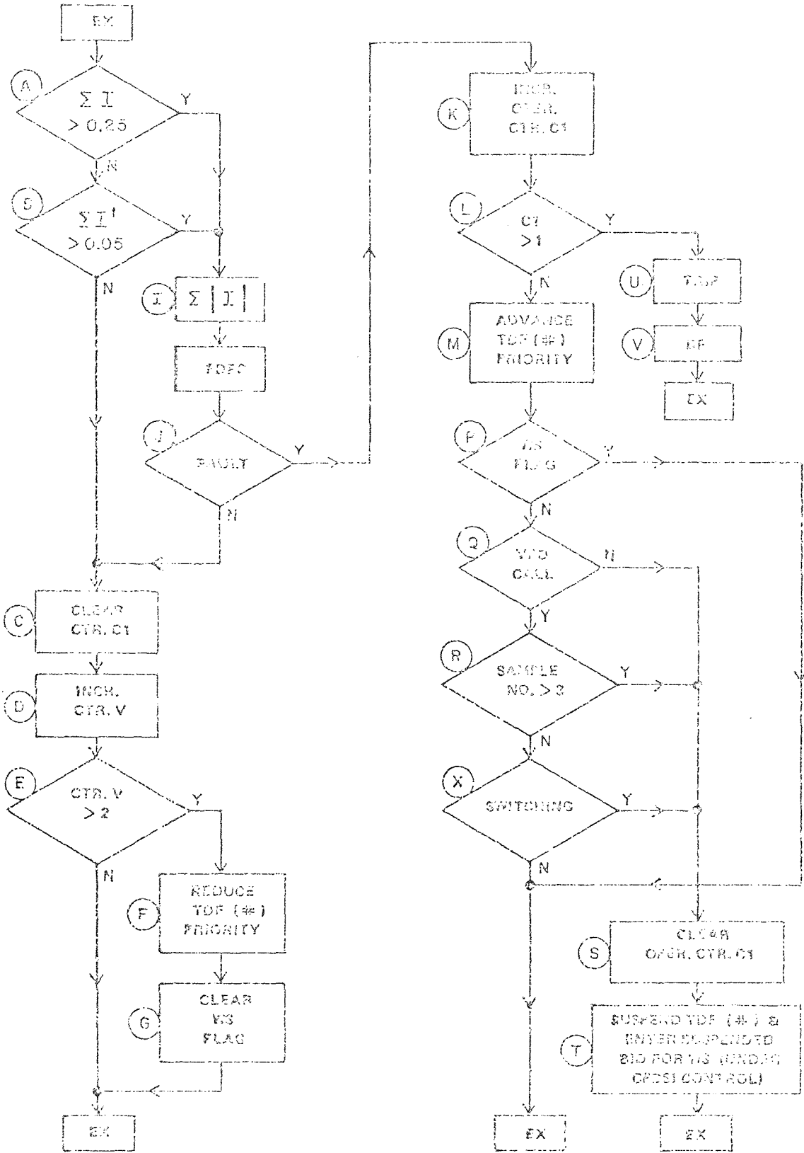
FIG. 25. TDF TRANSFORMER DIFFERENTIAL.
