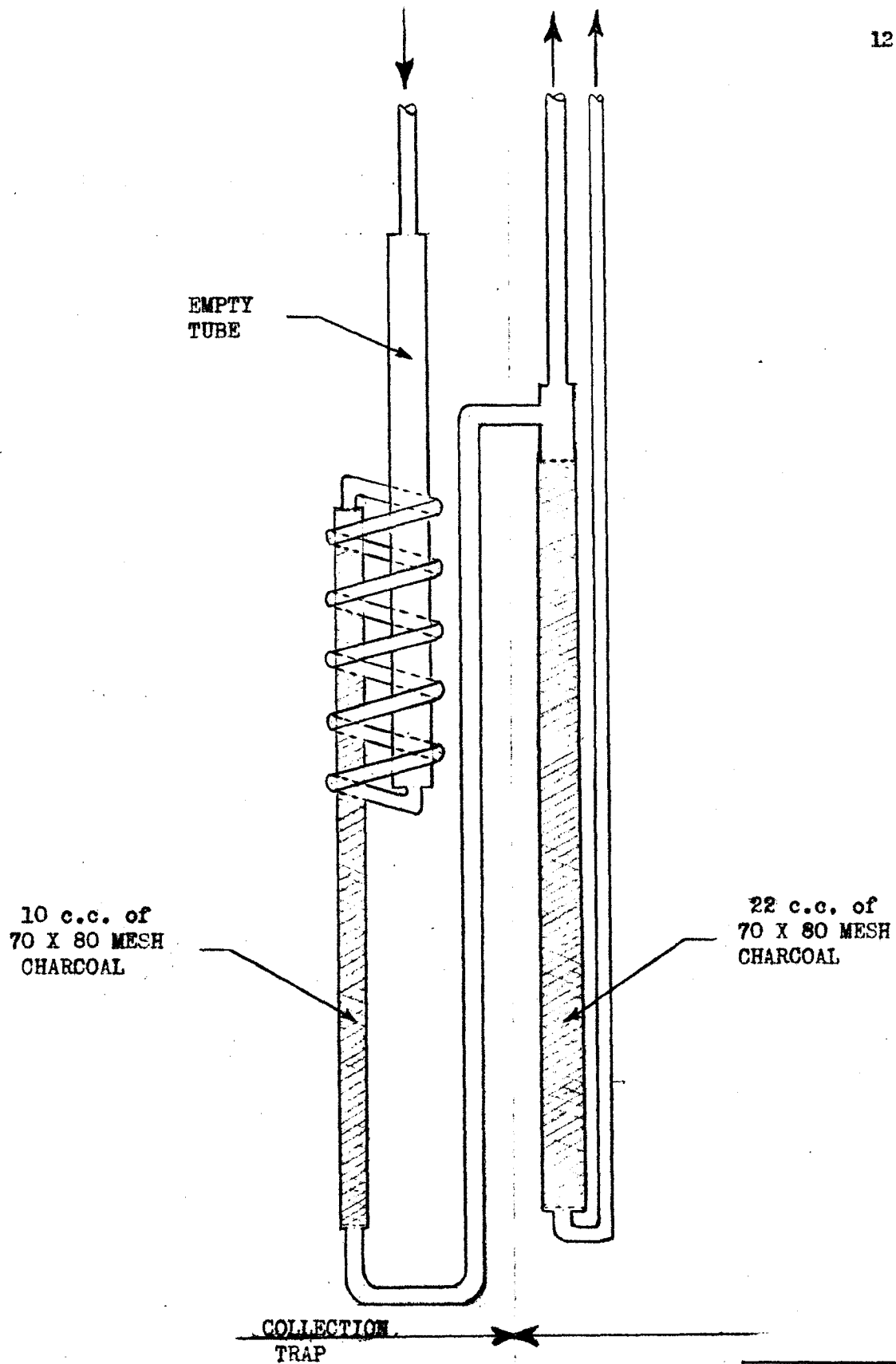
FIGURE III THE ELUTION COLUMN MATERIAL: COPPER & BRASS TUBING SILVER SOLDER CONNECTIONS SCALE 1/2" = 1"
