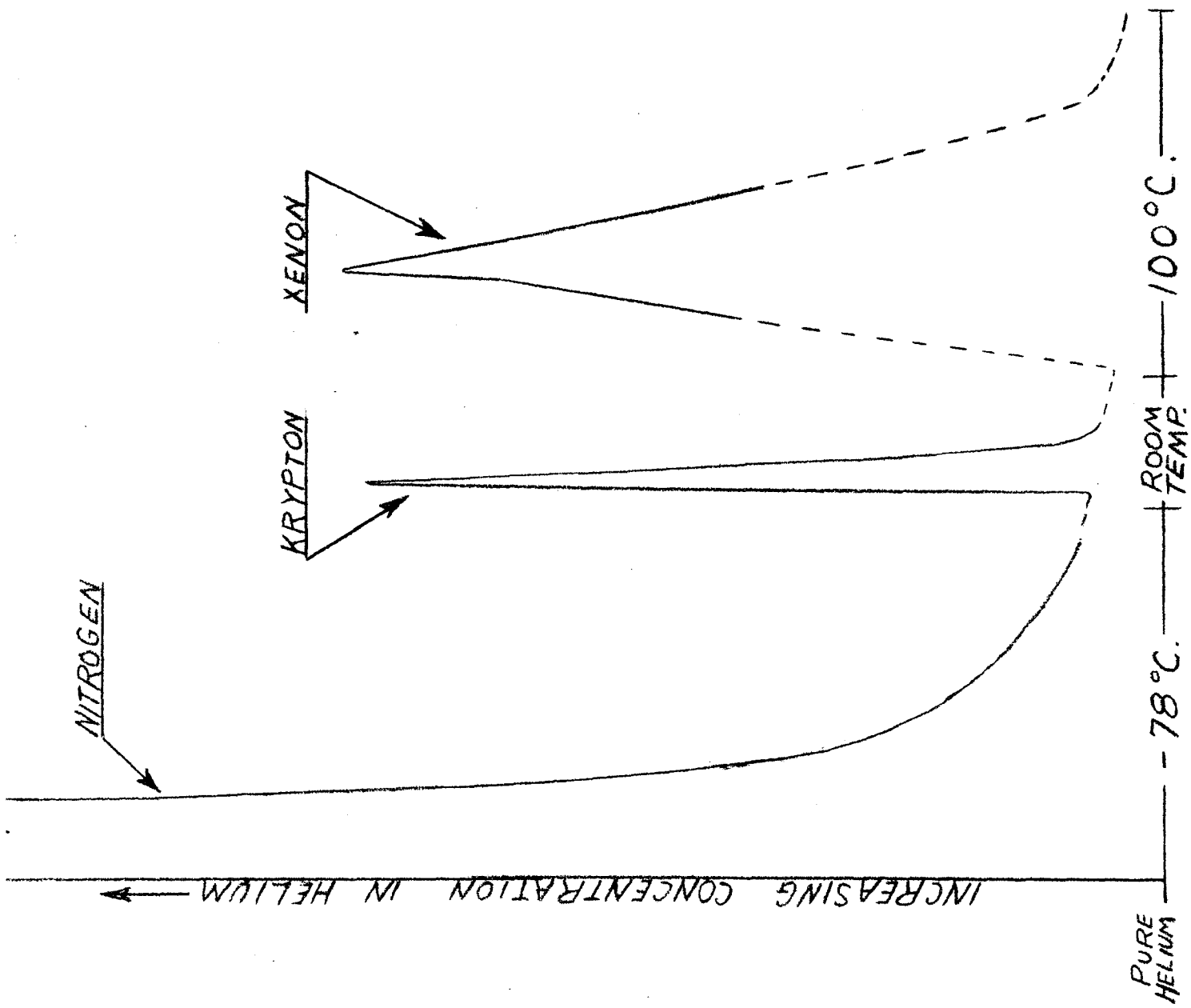
FIGURE VIII. THERMAL CONDUCTIVITY CURVE OF THE ELUTION OF NITROGEN , KRYPTON AND XENON AT THEIR RESPECTIVE TEMPERATURES.
