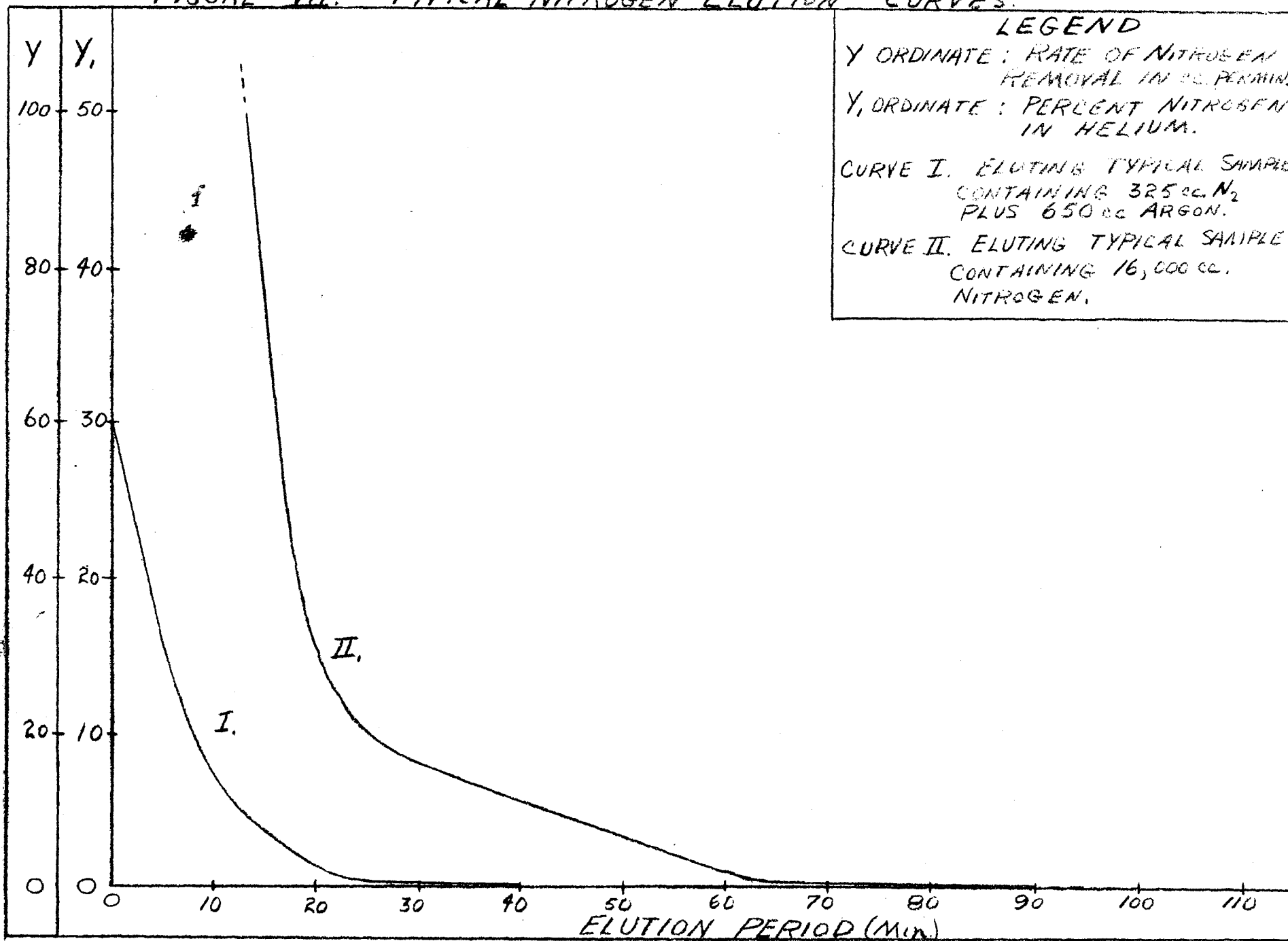
FIGURE VII. TYPICAL NITROGEN ELUTION CURVES.
