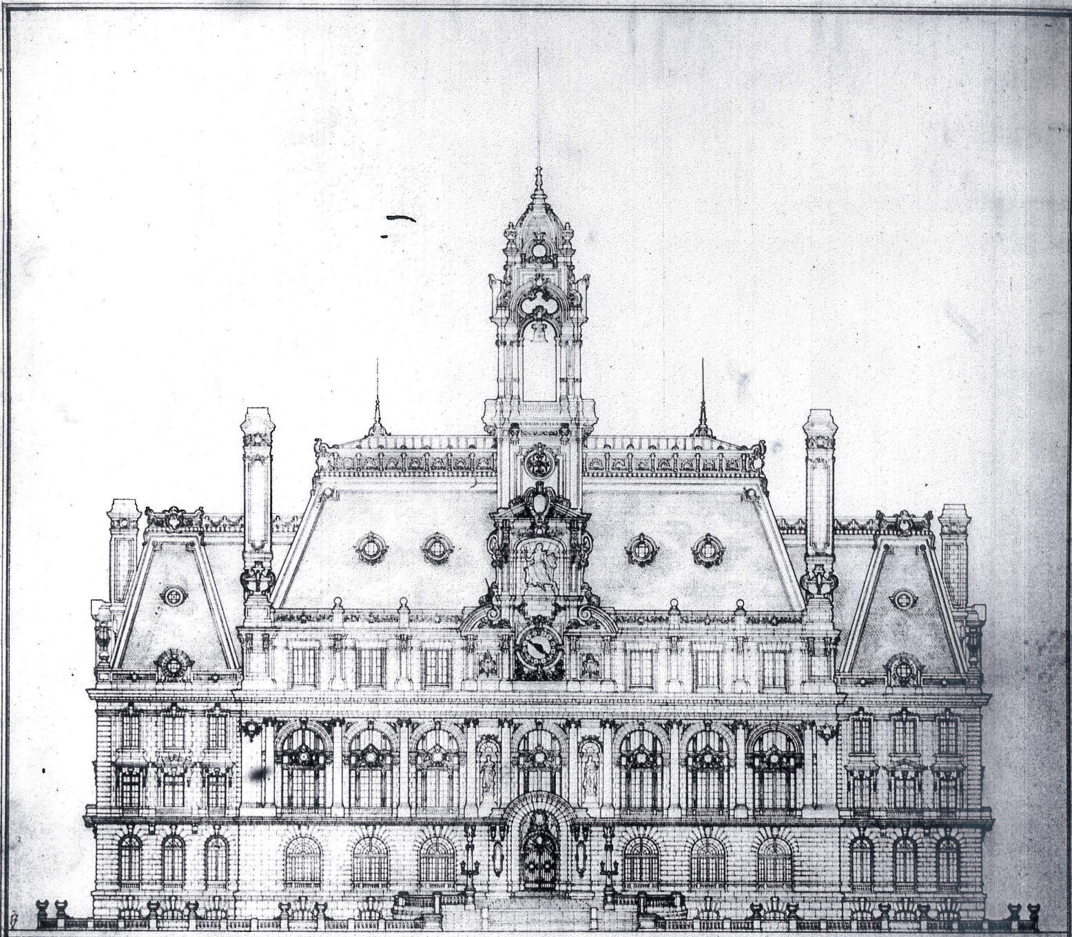
CITY HALL. FOR NEWARK N.J. FRONT ELEVATION. SCALE 1/8"=1'-0"
